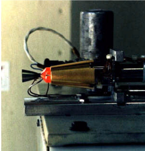
1-lbf, HAN-glycine monopropellant thruster firing.
