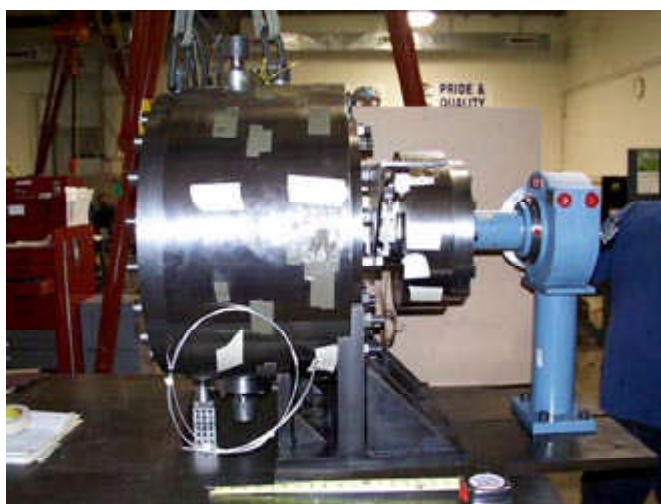
High-Temperature Seal Rig fabrication complete.
