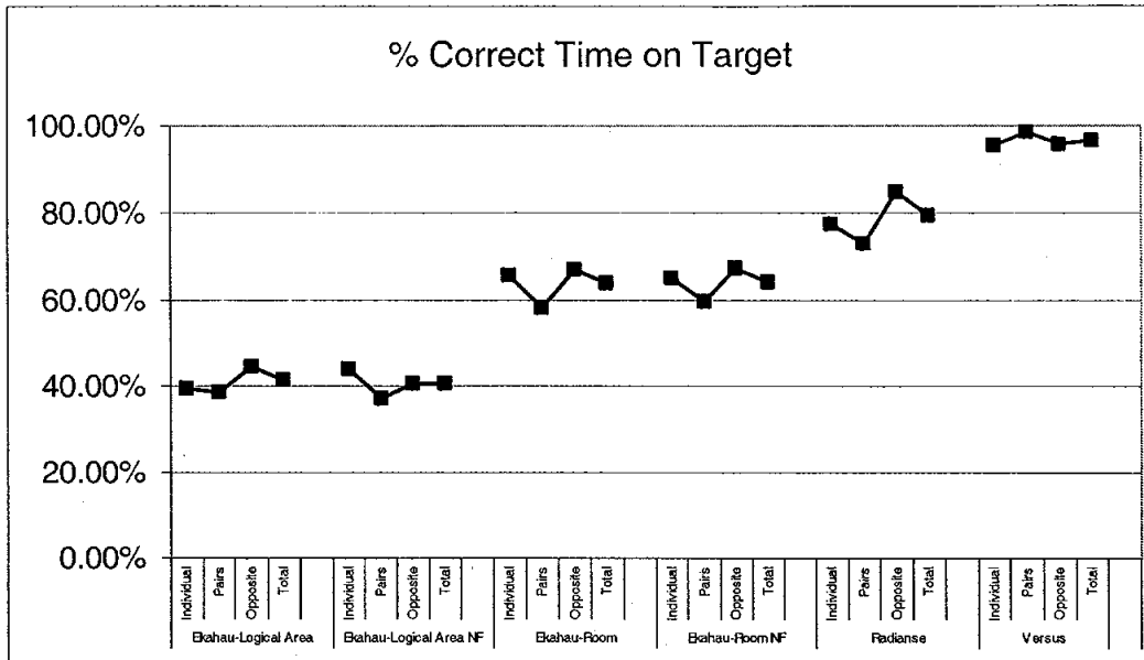
Figure 3: Percentage of time a system detected correctly by system and by condition
