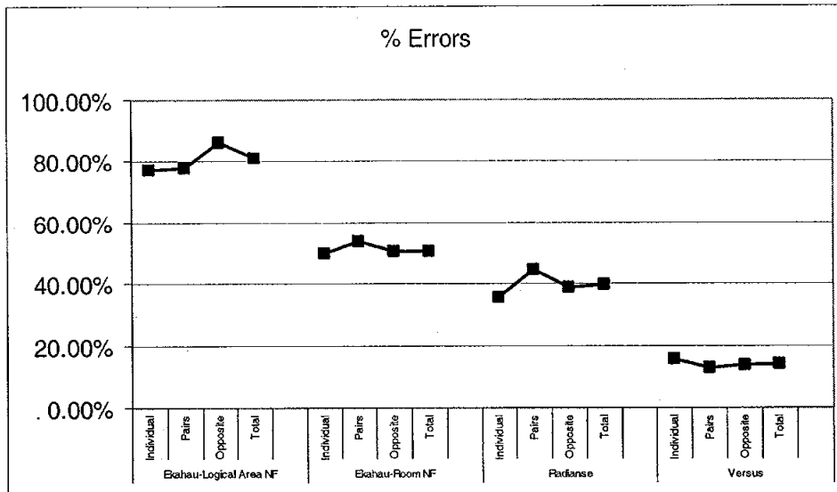
Figure 2. Percentage of error by system and by condition
