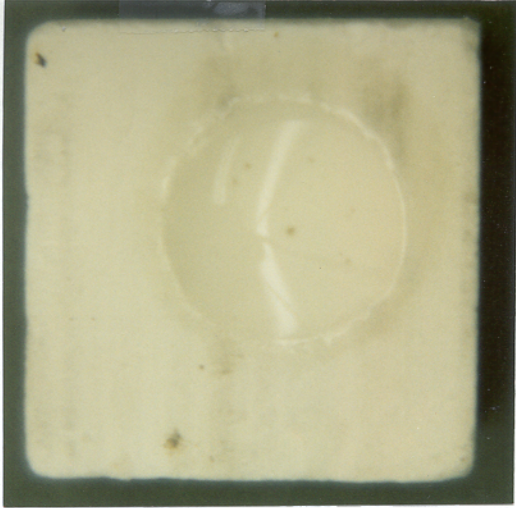
6. Photograph of phenyl methyl silicone mixed in air and dispensed in air into 1-inch pit in tile core on zero net-gravity turntable.
