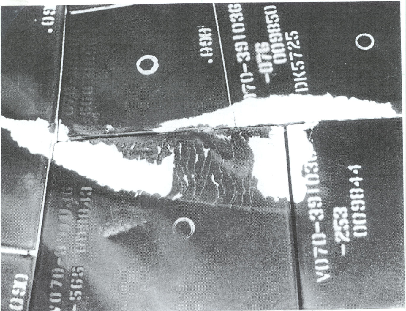
3. Impact damage in HRSI (TPS tile), right hand forward chine, STS 49.
