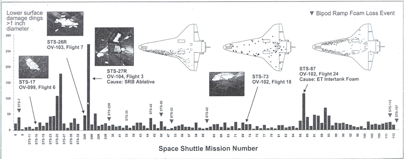
2. This chart shows the number of dings greater than one inch in diameter on the lower surface of the Orbiter after each mission from STS-6 through STS-113.
