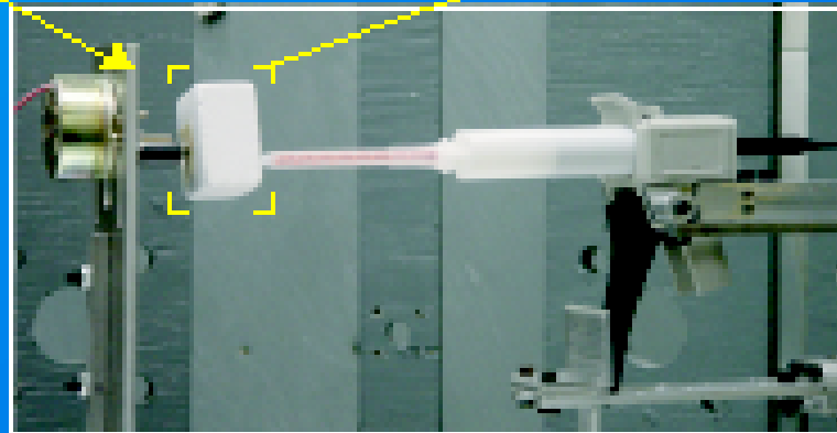
Microgravity Jig Inside Vacuum Chamber
