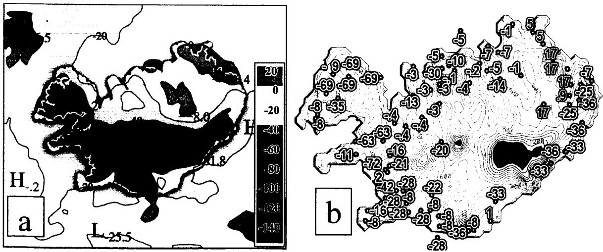
Figure 3.6. (a) Annual precipitation trend in Iceland simulated by Polar MM5 from 1991 to 2000 in mm/year, (b) Annual observed precipitation trend (mm/year) in Iceland for 1991-2000.
