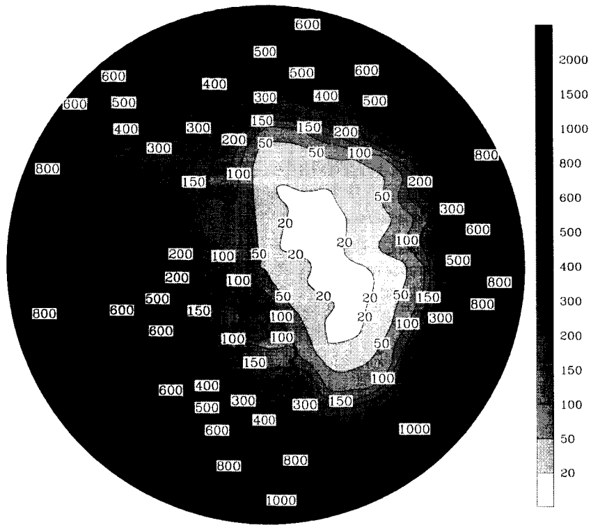
Figure 5.9 Mean annual precipitation produced by NCEP2 for the years 1979–99 ( \text{mm yr}^{-1} water equivalent).
