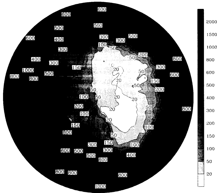
Figure 5.10 The mean annual precipitation produced by ECT for the years 1991–99 ( \text{mm yr}^{-1} water equivalent).
