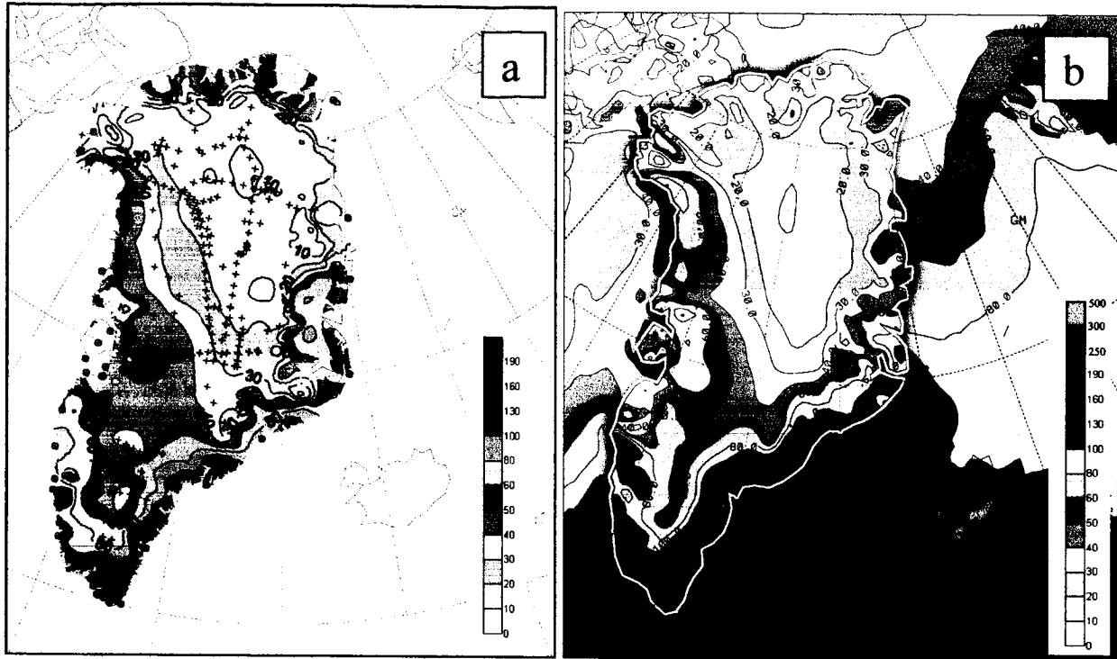
Figure.2.2 (a) Observed annual mean accumulation (cm/year water equivalent) from 1950 to 2000 ( from ice cores, coastal weather station and AWS data) and (b) the annual mean precipitation (1991-2000) simulated by Polar MM5 V3.5 (units: cm/year).
