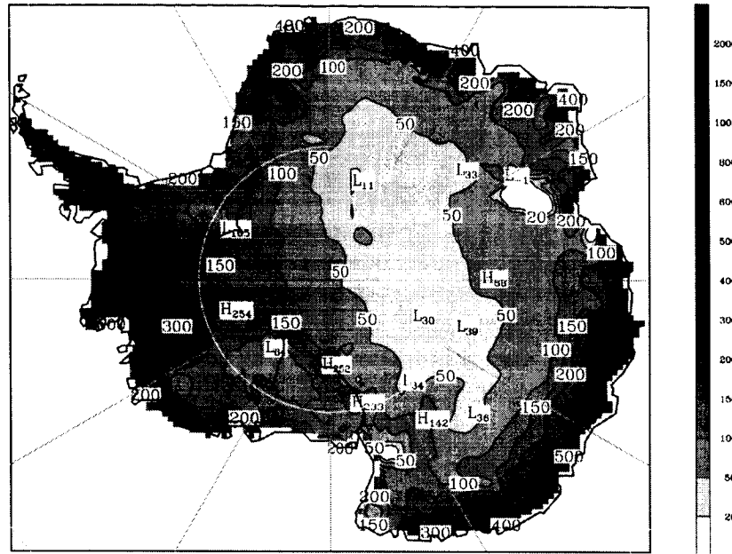
Figure 5.1 Vaughan et al. (1999) long-term accumulation distribution (mm yr -1 water equivalent).
