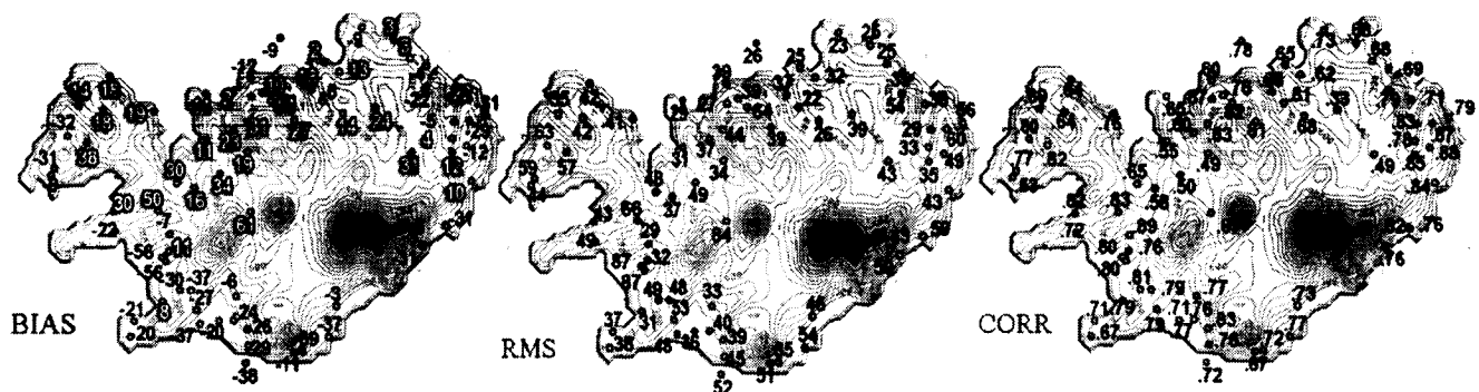
Figure 3.2. The monthly mean precipitation bias, RMS and correlation between observed and simulated by Polar MM5 from 1991 to 2000 for precipitation (mm). Terrain is shaded for reference; contour interval is 200m. Positive bias values are highlighted.
