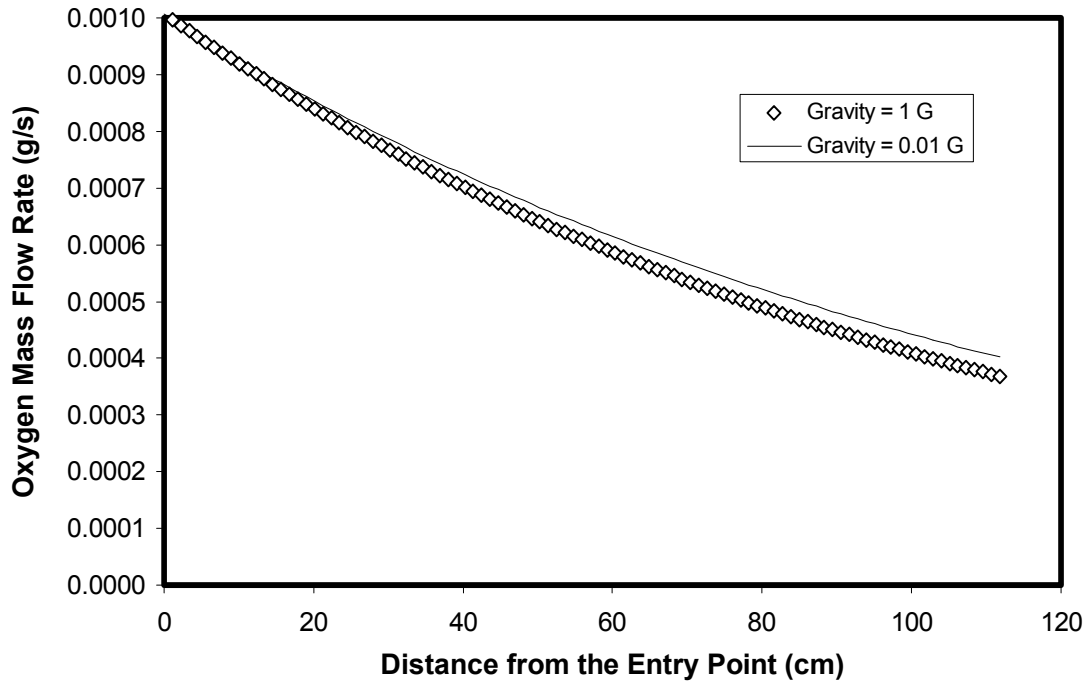
Figure 1 – Model-Calculated oxygen mass flow rate under 1-G and 0.01-G conditions
