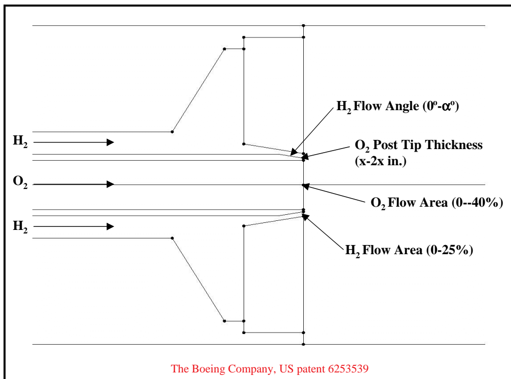
Figure 2. Independent Variables for Element Optimization.
