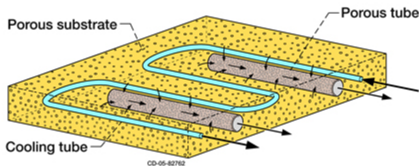
Condensing heat exchanger design concept based on composite porous media.
