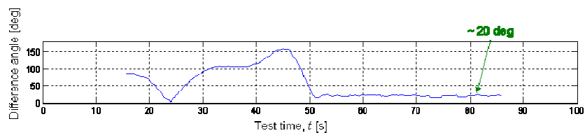
Figure 16: Angle between body z -axes of the two satellites during “relative search” test
