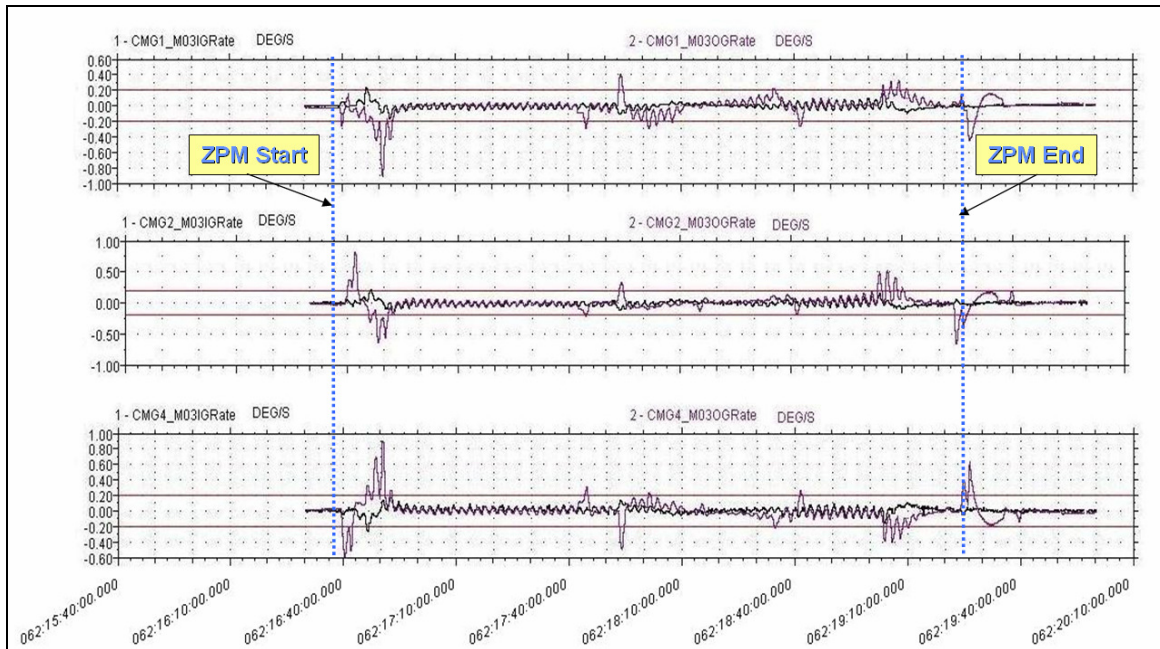
Figure 9. ZPM Flight CMG gimbals rates.
