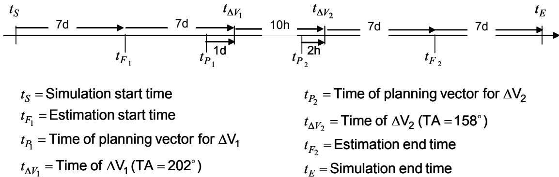
Figure 4: Simulation Timeline
