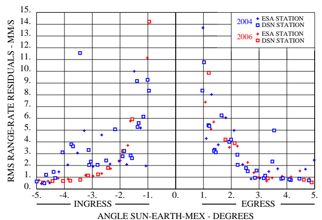
Fig. 7. MEX rms range-rate residuals in 2004 and 2006
