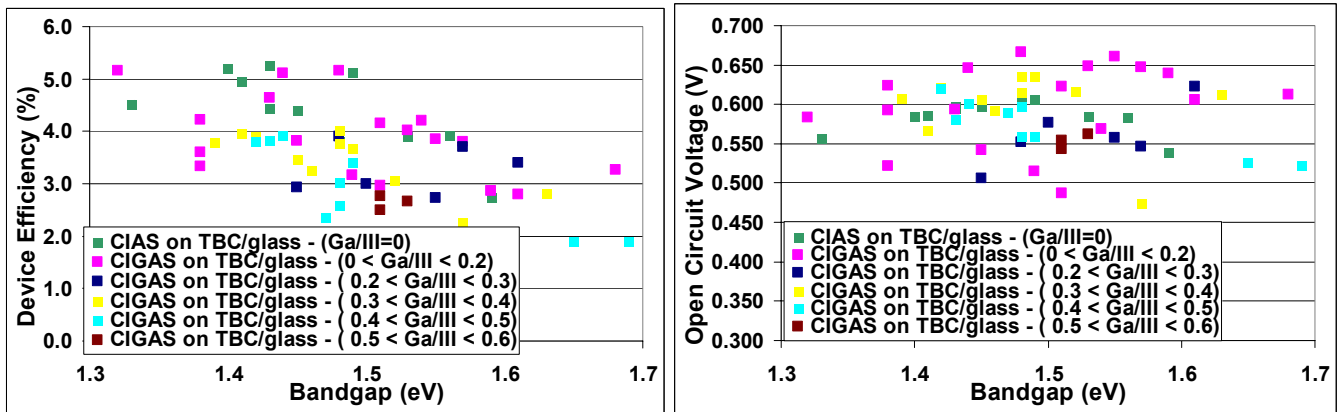
Figure 3 – Recent CIAS and CIGAS device efficiency (left) and open circuit voltage or Voc (right) versus bandgap and Ga content (Al content). Transparent back contact (TBC) device results shown only.
