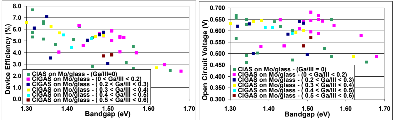
Figure 2 – Recent CIAS and CIGAS device efficiency (left) and open circuit voltage or Voc (right) versus bandgap and Ga content (Al content). Mo back contact device results shown only.
