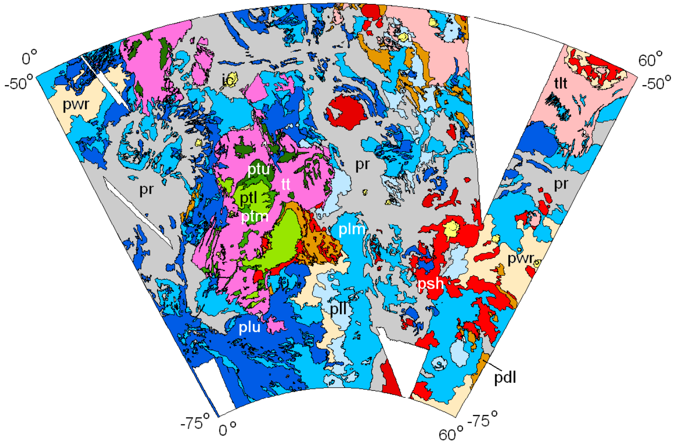
Fig. 1. Geological map of V-56 Lada Terra quadrangle. See table 1 for names of material units. Deformational structures are not shown here; these are currently being drawn on a separate map.
