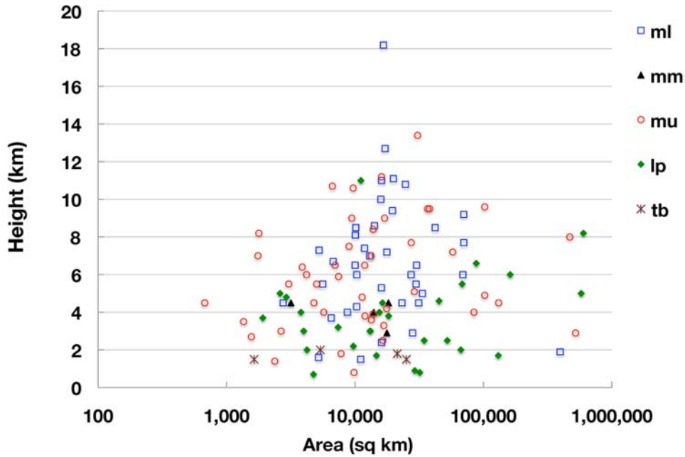
Figure 1. Plot of area-height relationships of Io's mountains. Mottled mountains (mm) are generally less high than lineated mountains (ml), consistent with their degradational formation. Undivided mountains (mu) are widely distributed, as lack of resolution inhibits better characterization. Tholi (volcanic mountains, tb) are of low relief, consistent with formation from low-viscosity lavas. Layered plains (lp) are mostly <6 km high, consistent with highly degraded mountains, grading into eroded plains (i.e., 'resurfacing' by mass wasting, a minor process on Io).
