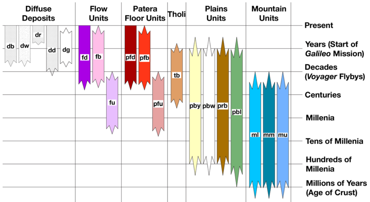
Figure 2. Correlation of exposed map units on Io. Symbols: ml, lineated mountains; mm, mottled mountains; mu, undivided mountains; pby, yellow bright plains; pbw, white bright plains; prb, red-brown plains; pbl, layered plains; tb, bright tholi; pfd, dark patera floors; pfb, bright patera floors; pfu, undivided patera floors; fd, dark flows; fb, bright flows; fu, undivided flows; db, bright diffuse deposits; dw, white diffuse deposits; dr, red diffuse deposits; dd, dark diffuse deposits; dg, green diffuse deposits.
