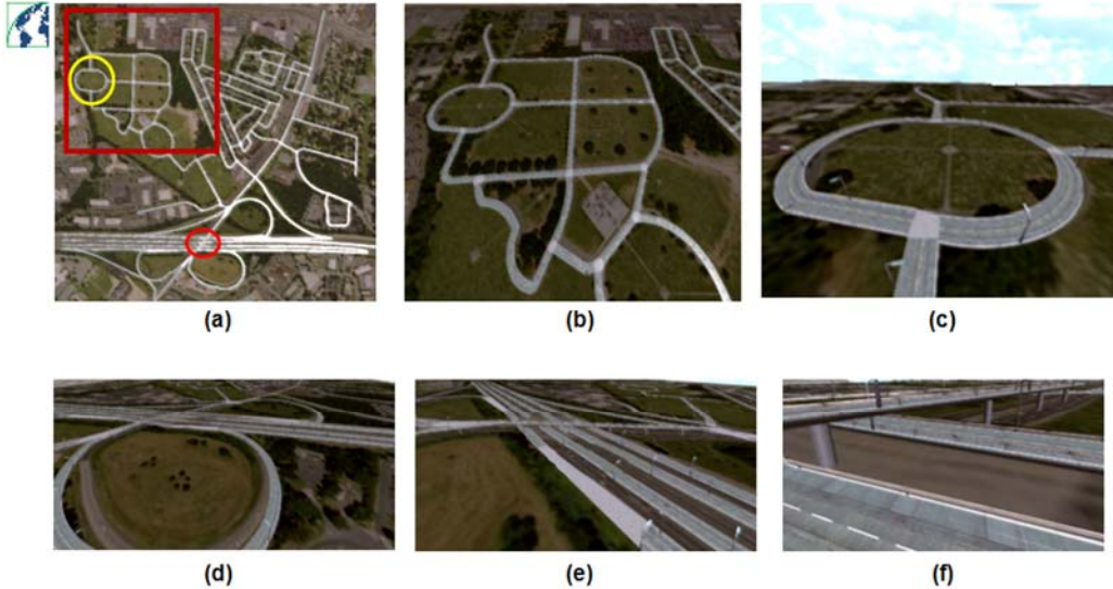
Figure 4. Experimental results (a) 3D road network generated for the exemplified road network. (b) Top view of the area indicated by the red rectangle in (a). (c) Side view of the area indicated by the yellow circle in (a). (d)(e)(f) Different views of the interchange part of the generated 3D road network model.
