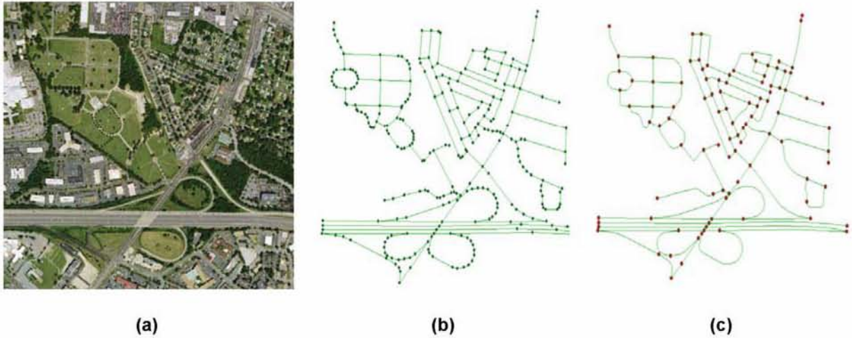
Figure 1 A road network example which contains several road segments, road intersections and a traffic interchange. (a) Satellite photo around VA-403 Norfolk, VA from USGS. (b) Road centerline and discrete road centerline points from road GIS data shown in ArcGIS for the same area. (c) Road network after topology extraction with extracted nodes indicated by red points.
