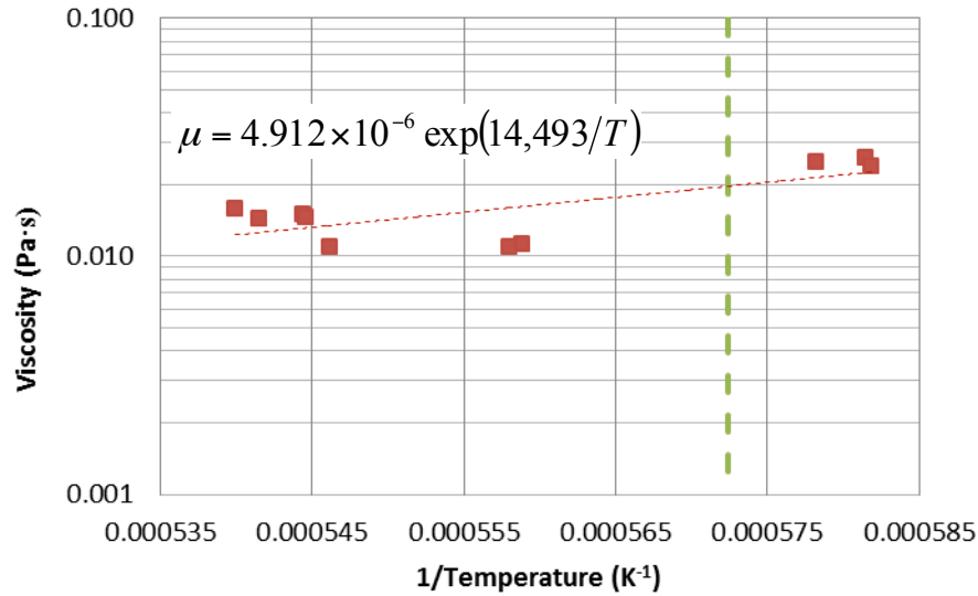
Figure 5. Variation of viscosity as a function of temperature.
