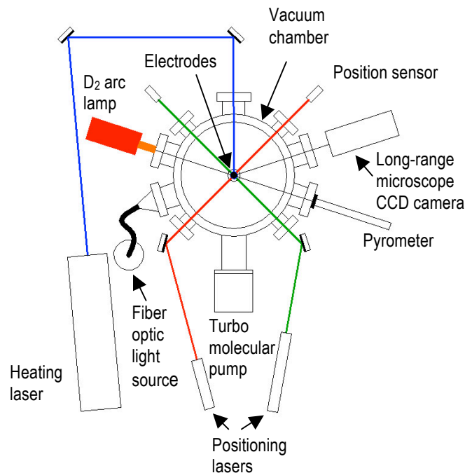
Figure 2. A schematic of ESL apparatus in NASA MSFC.
