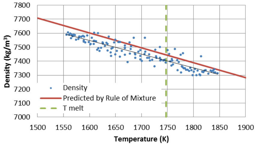
Figure 4. Variation of density as a function of temperature. The black line is a least-squares line fit to the measurements.
