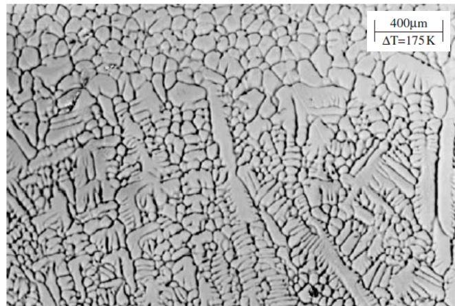
Figure 1. Microstructure of steel alloy: The solidification proceeded from top to bottom. The upper portion of the figure underwent double recalescence and thus shows globular and fine microstructures. As the solidification proceeded, the stable phase overtook the metastable solidification resulting in the dendritic structure shown in the lower portion of the figure. This corresponds to single recalescence behavior.
