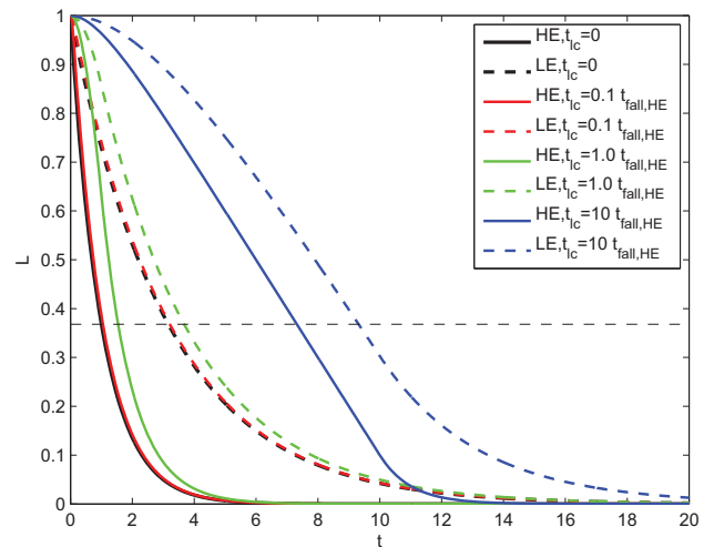
FIG. 4.— Exponentially decaying light curves of a flare in the MT. High and low energy luminosities ( \epsilon_{HE}/\epsilon_{LE} = 10 ) are plotted (normalized to 1) for increasing t_{lc} . Solid lines represent \epsilon_{HE} and dashed lines \epsilon_{LE} . Colors represent t_{lc} at differing factors of t_f , where t_{f,HE} is normalized to 1. The dashed black line is the 1/e decay time.
