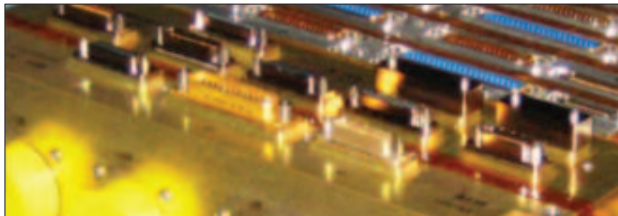
Figure 1. This picture shows the Design Concept , with the pedestals and the chassis as one piece of metal. The D-sub or Micro-D connector is then mounted on the pedestal. This pedestal provides a few extra millimeters for the conductive tape to make contact with the chassis.
