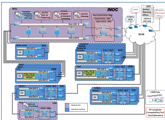
Fig. 3: Integrated Network Management (INM) System Architecture
