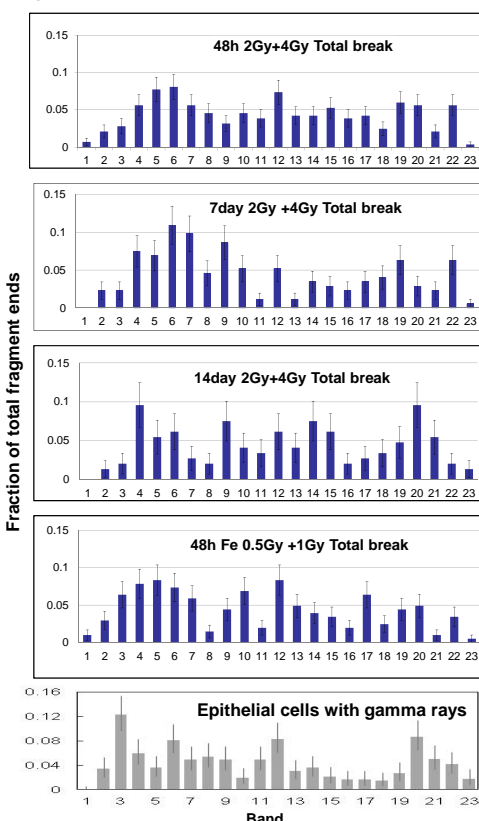
Fig. 8. Distribution for total chromosome ends
