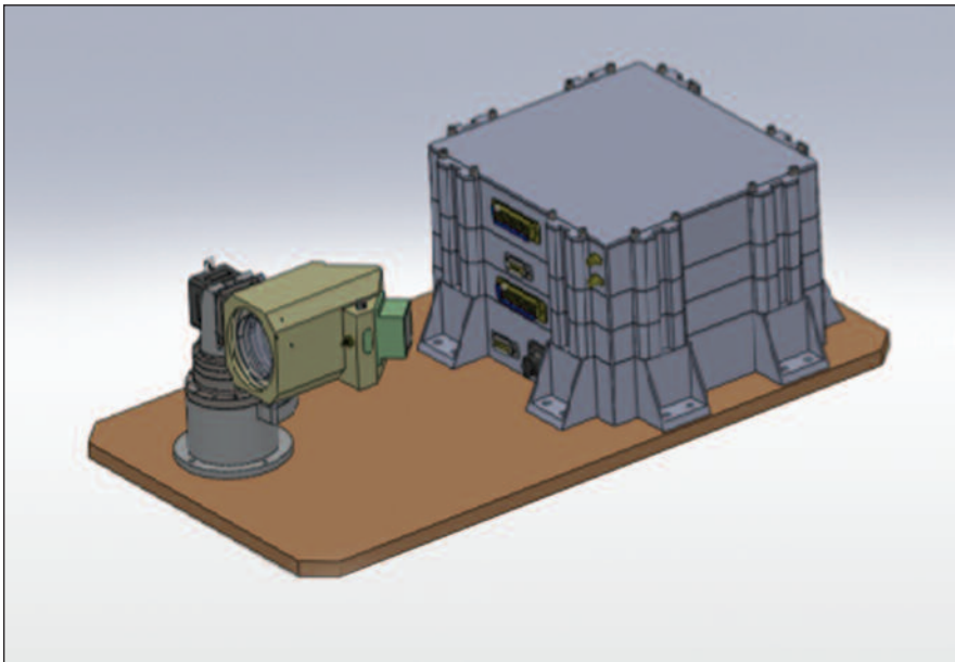
A Laser Communications Terminal consists of the optical head on a 2-axis gimbal (left), and an electronics/laser box (right).
