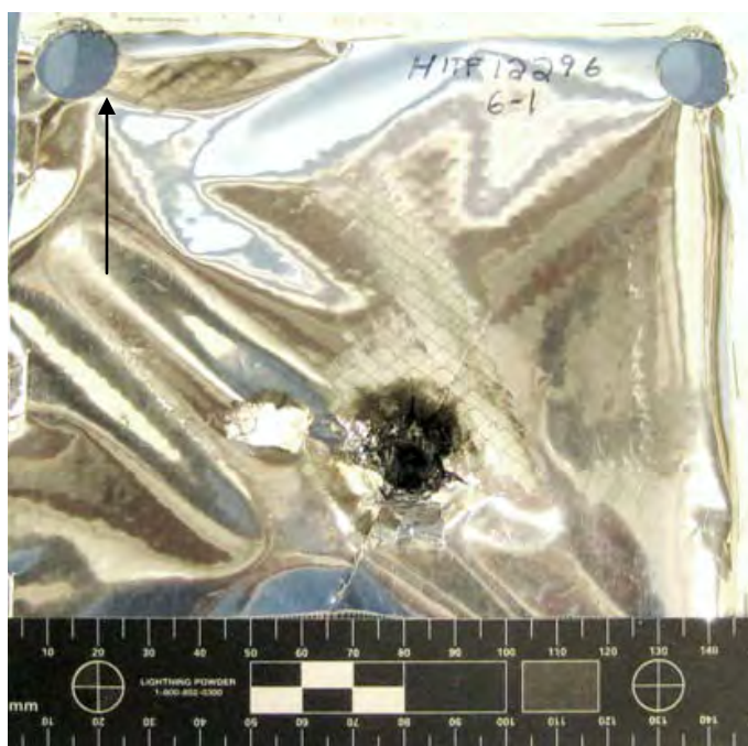
Figure 217 Overall View of Damage to Back Side of MLI (scale in 5mm increments / black arrow indicates flight path of projectile)
