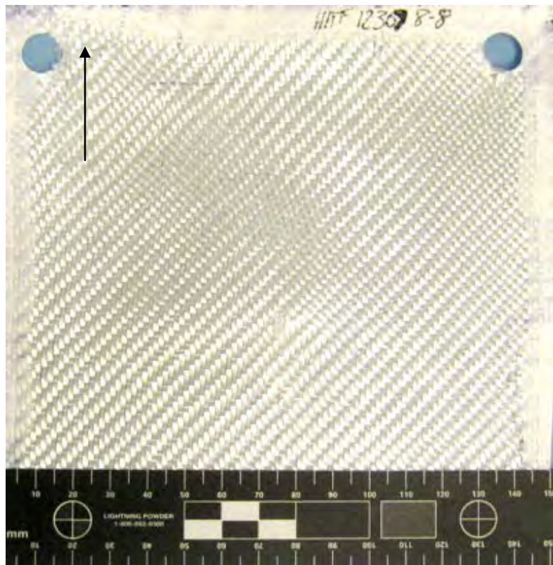
Figure 420 Overall View of Damage to Back Side of 8th Fiberglass Layer (scale in 5mm increments / black arrow indicates flight path of projectile)
