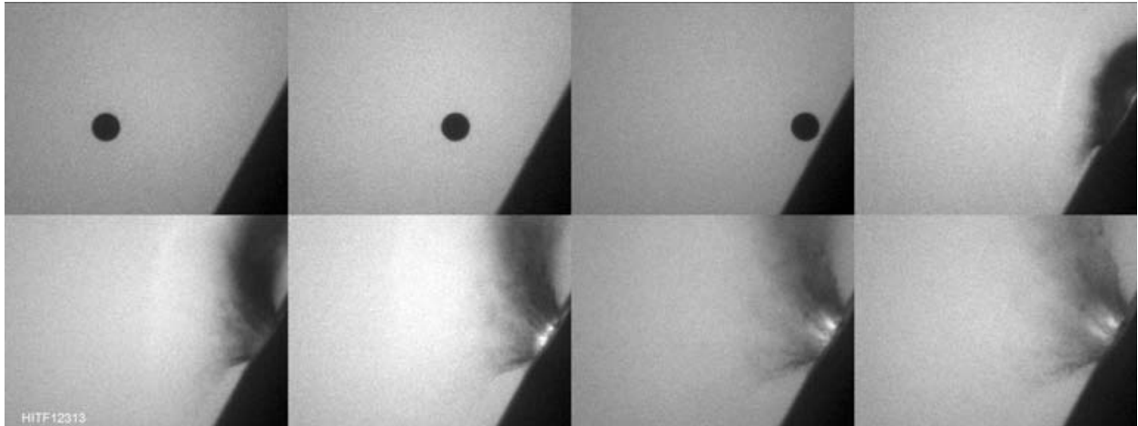
Figure C98 Projectile Captured Prior to Impact and Impacting Target (via SIMX-8 Camera)
