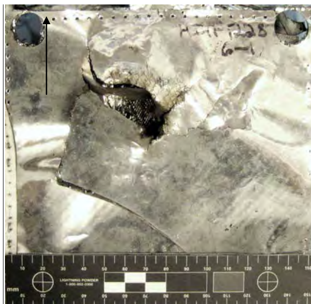
Figure 71 Overall View of Damage to Back Side of MLI (scale in 5mm increments / black arrow indicates flight path of projectile)
