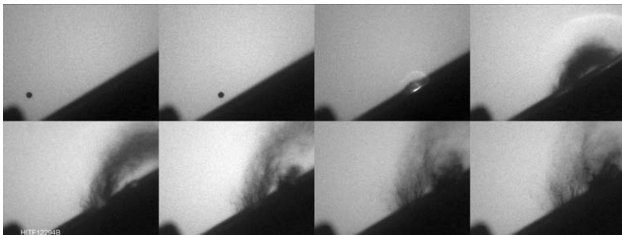
Figure C33 Projectile Captured Prior to Impact and Impacting Target (via SIMX-8 Camera)
