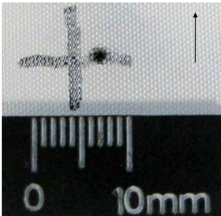
Figure 12 Close-up View of Damage to Front of MLI (scale in 1mm increments / black arrow indicates flight path of projectile)
