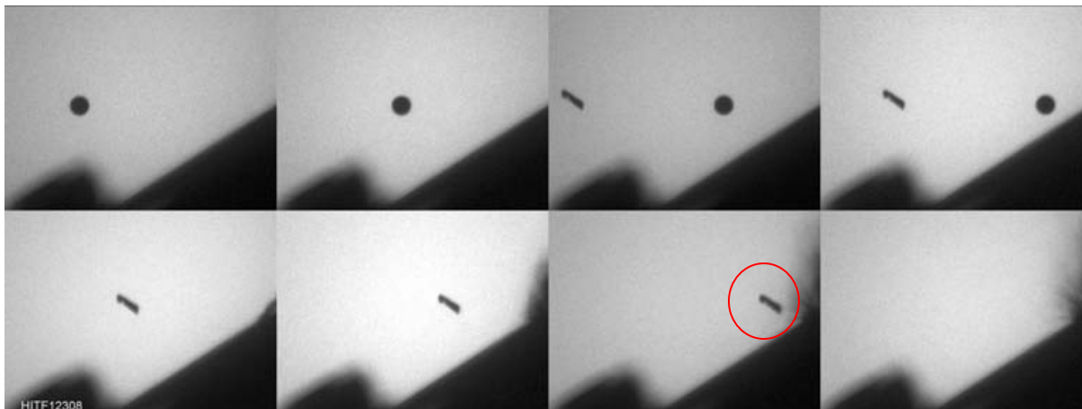
Figure C77 Projectile and Secondary Debris Captured Prior to Impact and Impacting Target (via SIMX-8 Camera / secondary debris within red circle)
