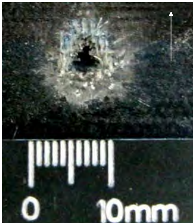
Figure 460 Close-up View of Damage to Front of NP 504 Substrate (scale in 1mm increments / white arrow indicates flight path of projectile)
