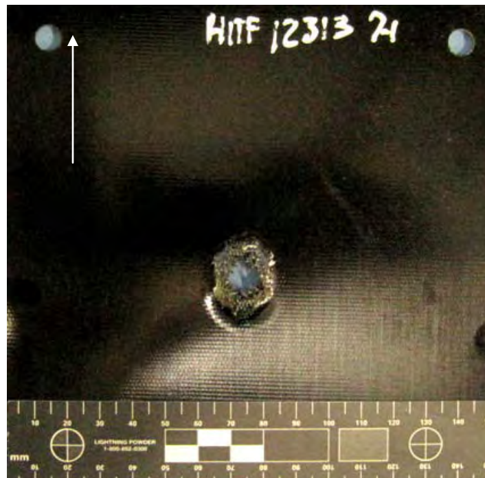
Figure 552 Overall View of Damage to Back Side of NP 504 Substrate (scale in 5mm increments / white arrow indicates flight path of projectile)
