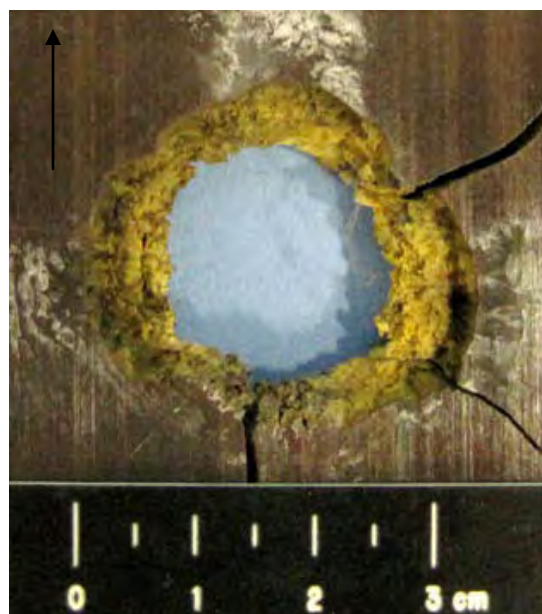
Figure 524 Overall View of Damage to Front of TORLON 5030 Delaminated from Substrate (black arrow indicates flight path of projectile / scale in 5mm increments)
