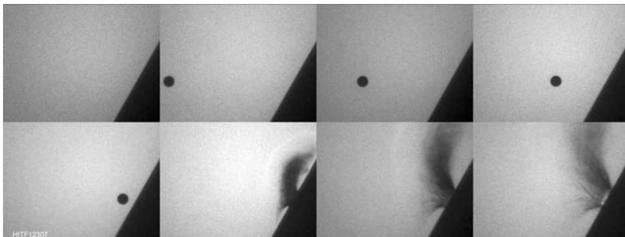
Figure C74 Projectile Captured Prior to Impact and Impacting Target (via SIMX-8 Camera)
