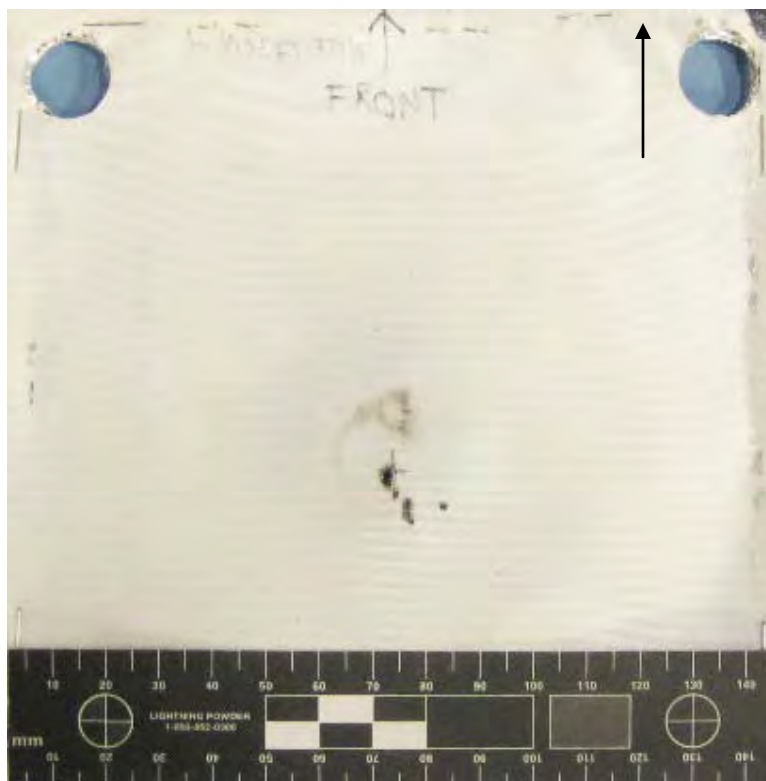
Figure 357 Overall View of Damage to Front of MLI (scale in 5mm increments / black arrow indicates flight path of projectile)
