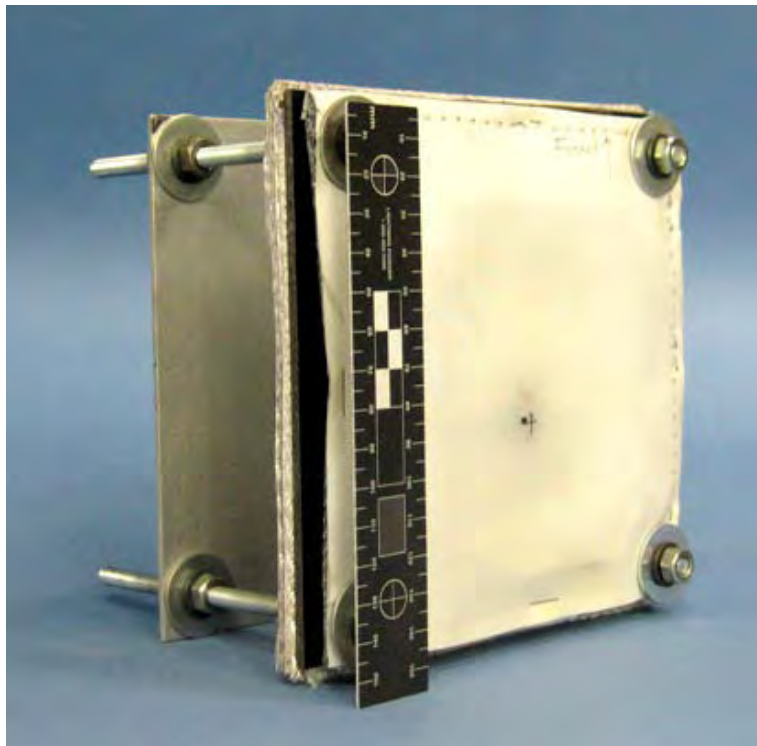
Figure 52 Overall Front Oblique View of Sample (scale in 5mm increments)
