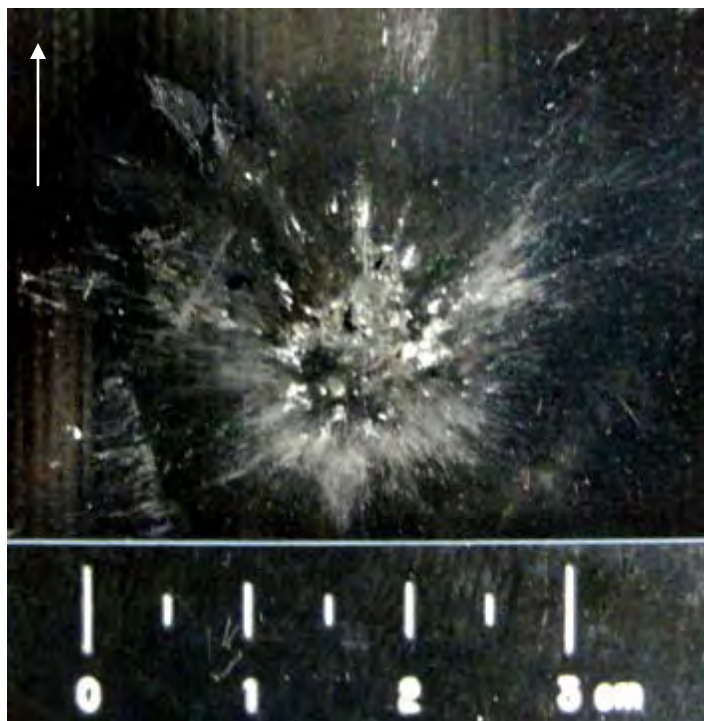
Figure 284 Close-up View of Damage to Front of NP 504 Substrate (scale in 5mm increments / white arrow indicates flight path of projectile)
