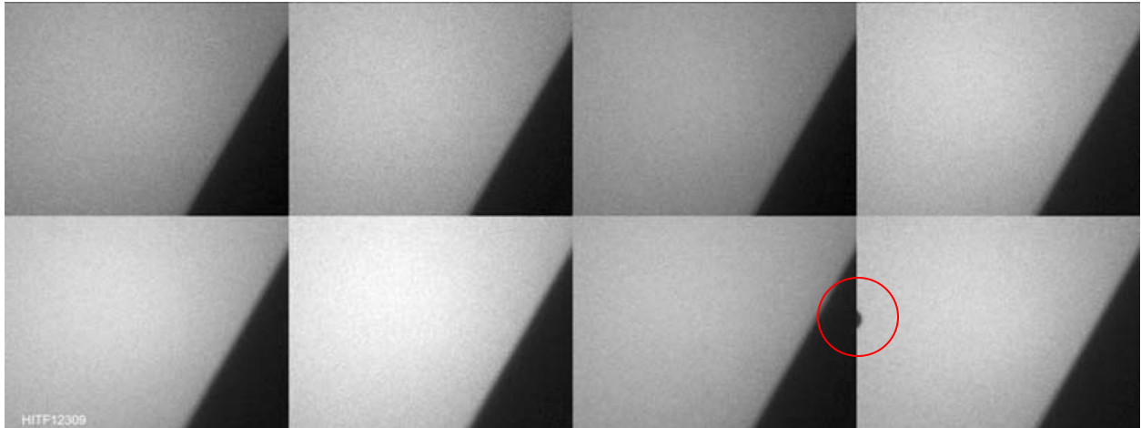
Figure C83 Partial Projectile Captured Prior to Impact (via SIMX-8 Camera / partial projectile within red circle)
