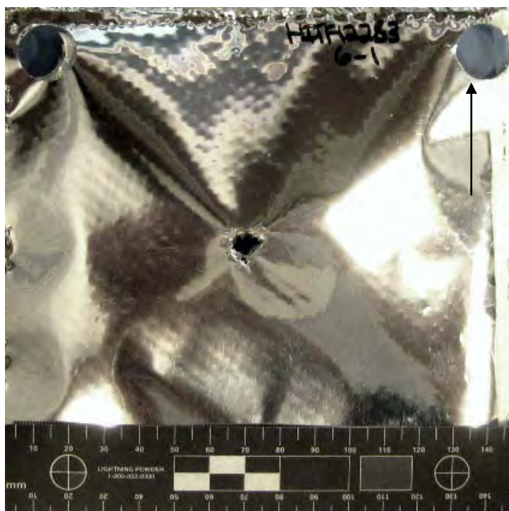
Figure 13 Overall View of Damage to Back Side of MLI (scale in 5mm increments / black arrow indicates flight path of projectile)
