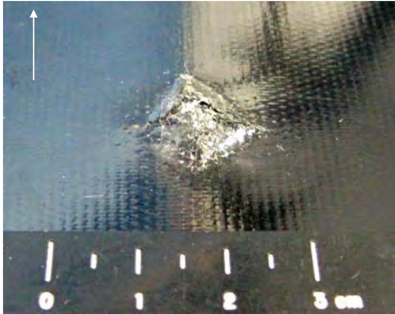
Figure 419 Close-up Oblique Side View of Damage to Back Side of NP 504 Substrate (scale in 5mm increments / white arrow indicates flight path of projectile)
