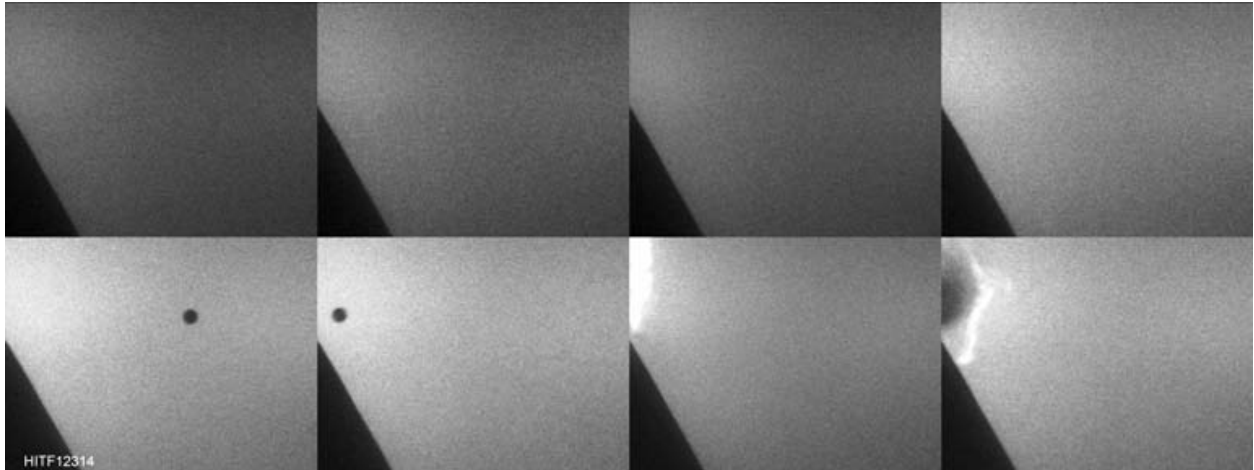
Figure C101 Projectile Captured Prior to Impact and Impacting Target (via SIMX-8 Camera)
