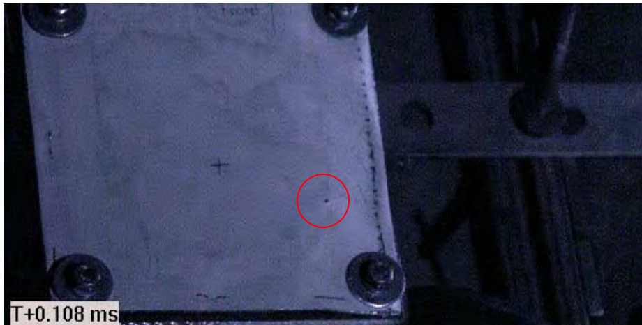
Figure C93 Image of Projectile Captured Prior to Impact (via Phantom v711 / projectile within red circle)
