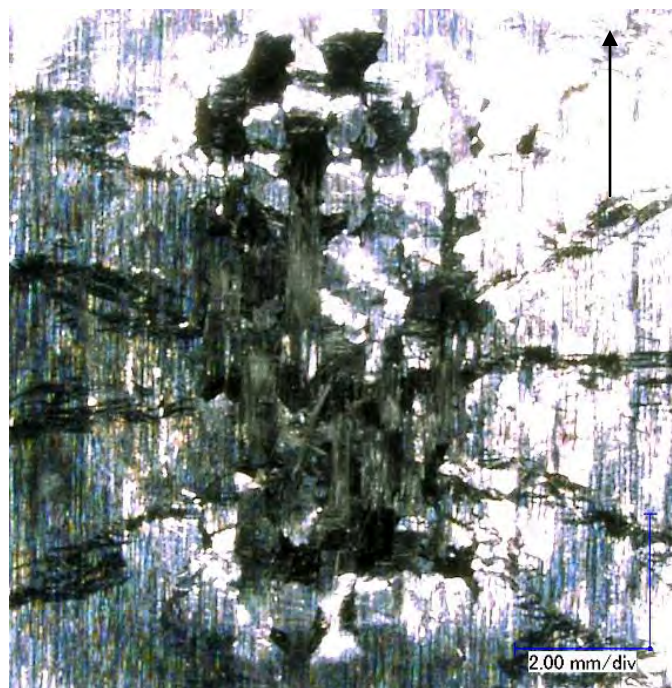
Figure 62 Close-up View of Most Significant Damage to Back Side of NP 504 Substrate (black arrow indicates flight path of projectile / damage within red circle in Figure 61)
