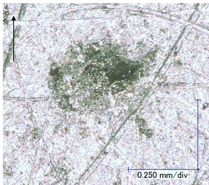
Figure 83 Close-up View of Most Significant Damage to Front of Rear Wall (black arrow indicates flight path of projectile / damage within red circle in Figure 82)
