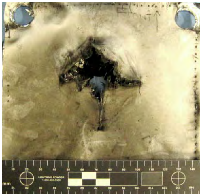
Figure 567 Overall View of Damage to Front of MLI (scale in 5mm increments / black arrow indicates flight path of projectile)
