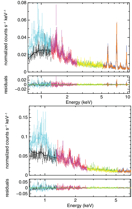
FIG. 2 (color online). Unabsorbed Suzaku XIS03 [top panel, (a)] and XIS1 [bottom panel, (b)] spectra of the Ursa Minor and Draco dwarf spheroidal galaxies (Draco has the greater low energy flux). The best joint-fit baseline models, that include both non-x-ray and astrophysical background components and residuals are also shown. The spectra are divided into segments spanning the following energies: 0.7–1.3 keV (Ursa Minor: black, Draco: light blue), 1.3–2.6 keV (Ursa Minor: red, Draco: magenta), 2.6–5.2 keV (Ursa Minor: green, Draco: yellow), 5.2–10.5 keV for XIS03 or 5.2–7 for XIS1 (Ursa Minor: blue, Draco: orange).
