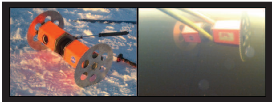
Figure 1. The JPL Buoyant Under-Ice Rover shown on the ice (left) and crawling on the underside of the ice (right) during a 2012 field campaign in Alaska. For scale, the rover is 0.54 m wide.
