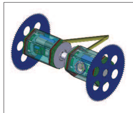
Figure 2. Computer aided design (CAD) model of the JPL Buoyant Under Ice Rover showing the two independent chassis regions each with wheel, camera, and instrument capability. The central tether spool can also operate independent of the side chassis.
