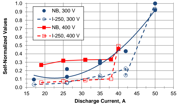
Figure 3 Comparison of corrected, I_{B, 250 \text{ nm}} , and normalized, N_B , values.
