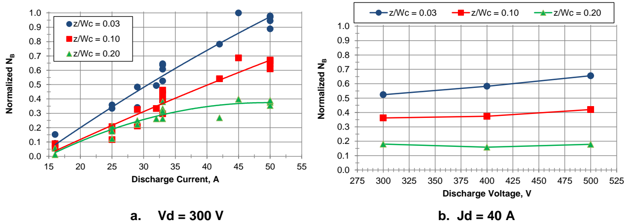
Figure 6 Comparison of N_B trends for three axial locations along the outer wall for V_D = 300 V and J_D = 40 A.
