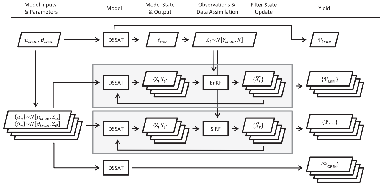
Figure 1. Observing system simulation experiment process diagram: Transparent gray boxes represent sequential importance resampling filter (SIRF) and ensemble Kalman filter (EnKF) assimilation algorithms, \mathbf{u} are forcing data, \mathbf{v} are model parameters, \mathbf{X} are model states, \hat{\mathbf{X}} are filter-updated model states, \mathbf{Y} are modeled leaf area index (LAI) and \theta , \mathbf{Z} are observed LAI and \theta , and \Psi is yield. \mathbf{R} , \Sigma_{\theta} , and \Sigma_{\mathbf{u}} are uncertainty variances listed in Tables 4 and 5 and equation (5a).
