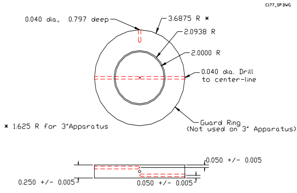
Figure 5 - Typical 0.250" specimen design.
