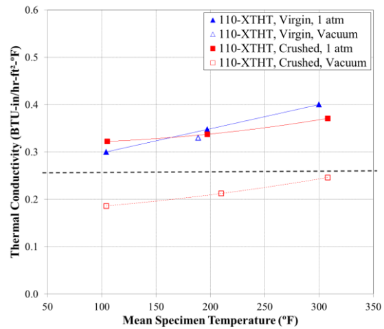
Figure 7: 110-XTHT thermal conductivity results.
