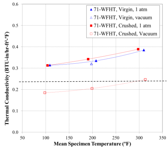
Figure 6: 71-WFHT thermal conductivity results.
