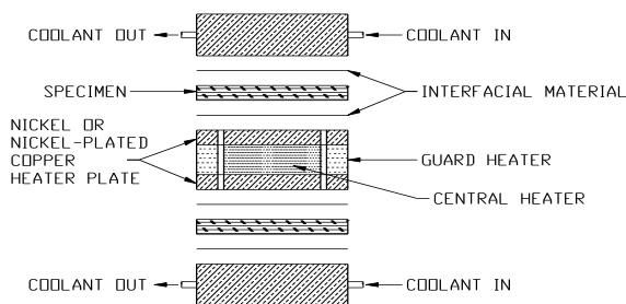
Figure 3 - Guarded hot plate apparatus schematic.
