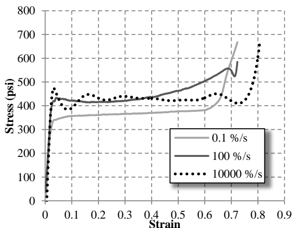
Figure 4-Mechanical properties of the 71-WFHT foam.
