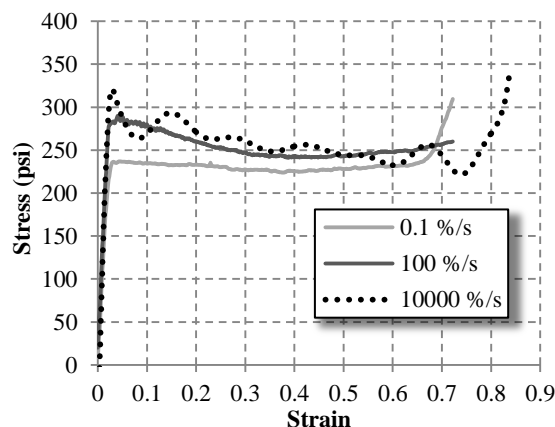
Figure 2 - Mechanical properties of the 110-XTHT foam.
