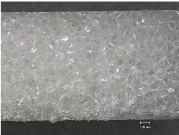
Figure 8 - Image of virgin 110-WFHT foam.
