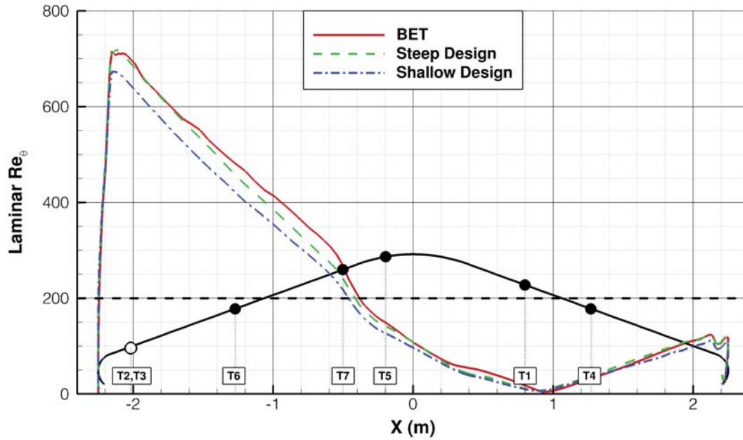
Figure 12. LAURA Laminar Re_\theta at Peak Heating on the BET and TPS Design Trajectories
