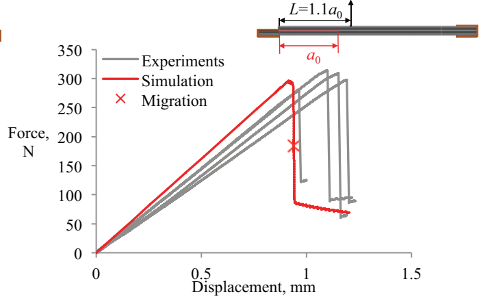
(b) load offset: L = 1.1a_0 ,
