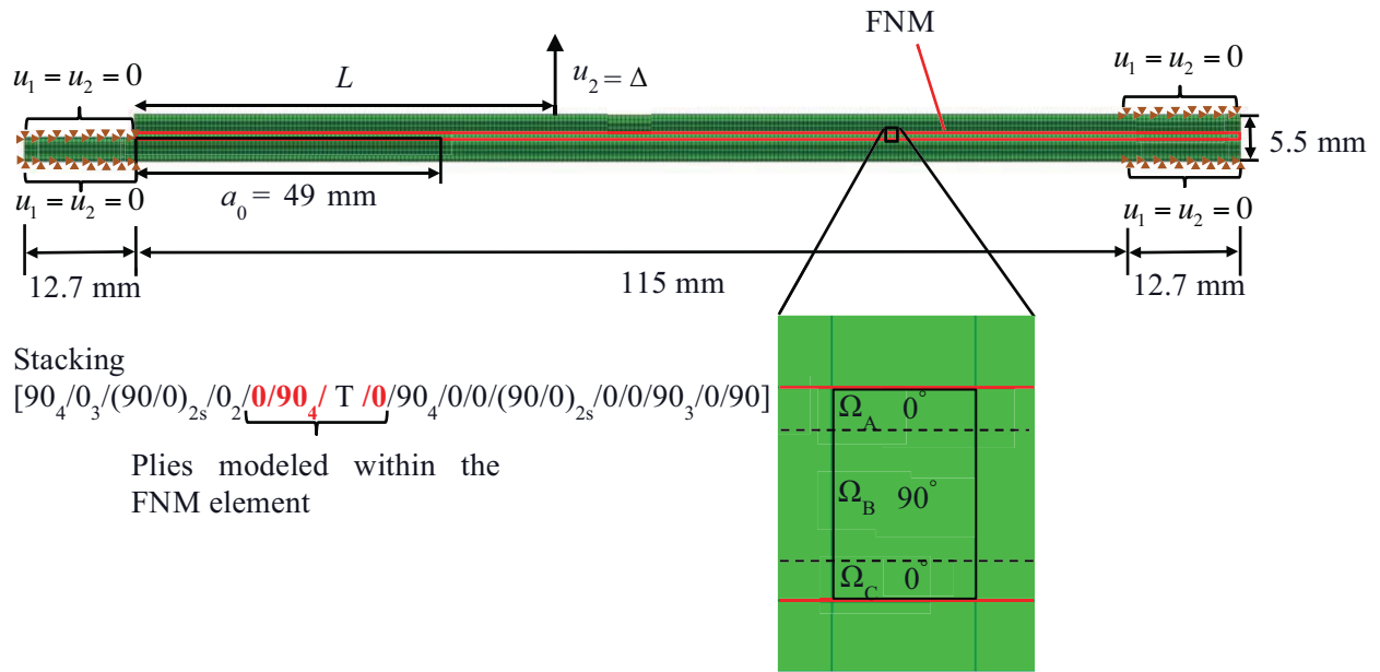
Figure 6. Finite element model, and boundary conditions of migration test specimen [7].
