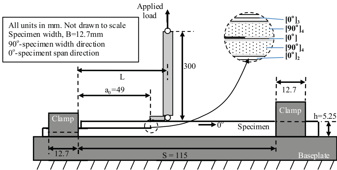
Figure 5. Schematic of delamination migration test configuration [7].
