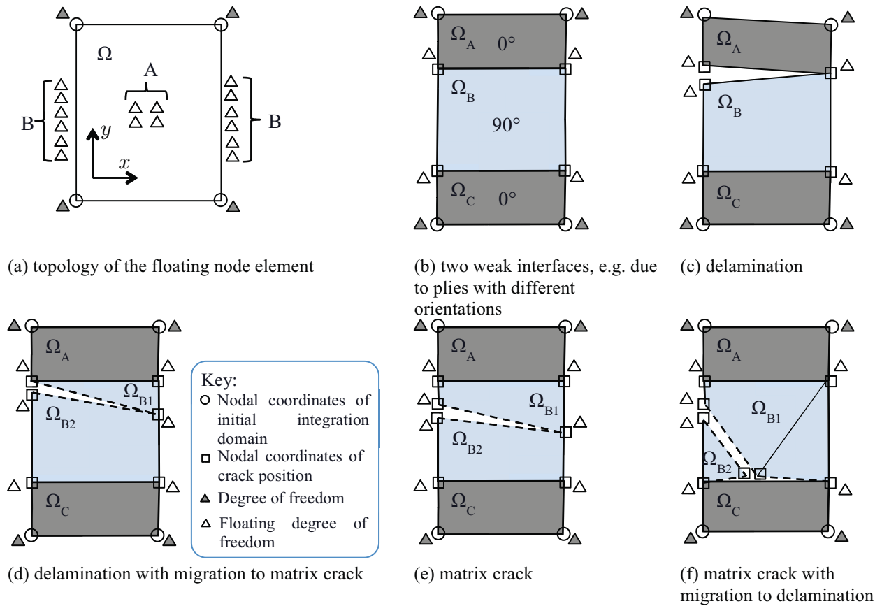
Figure 2. Floating node element used showing different weak/strong discontinuities scenarios
