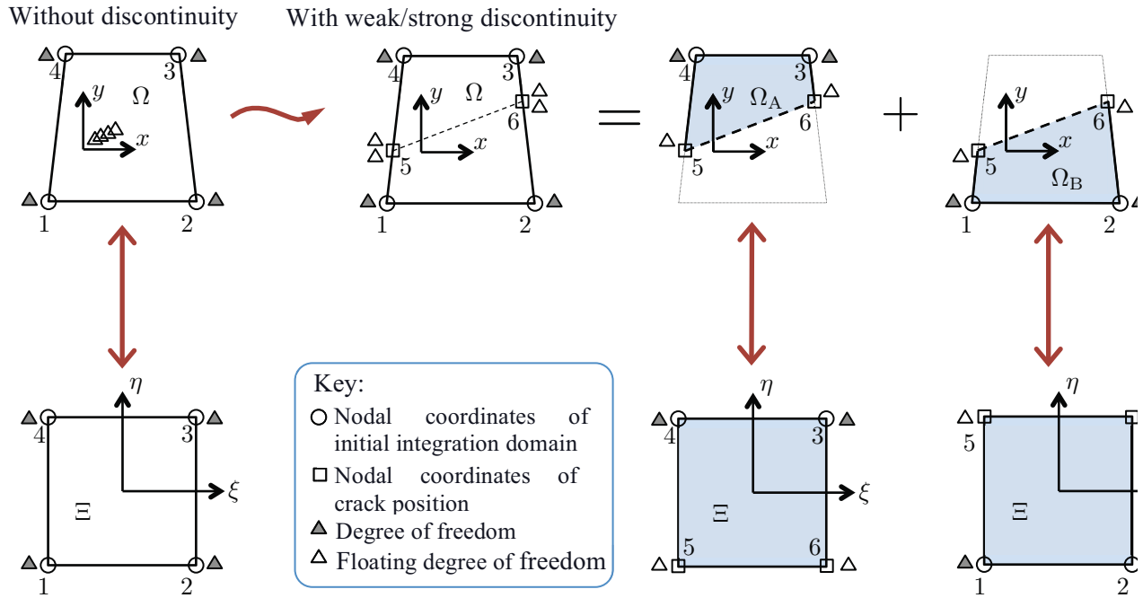
Figure 1. Overview of the Floating Node Method (FNM).
