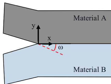
Figure 3. Virtual Crack Closure Technique and Floating Node Method for arbitrary crack propagation.
