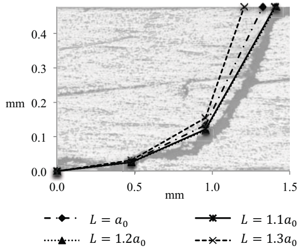
Figure 9. Comparison of experimentally observed crack path for L = a_0 , and simulated crack paths for different load-offsets, L .
