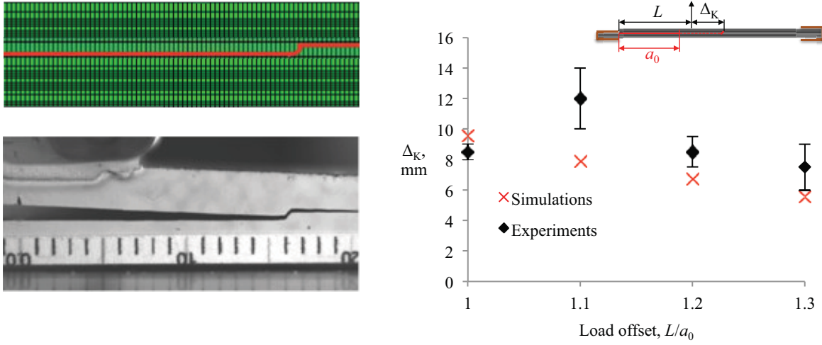
(a) qualitative comparison between simulated and experimental crack paths (b) variation of \Delta_K with normalized load offset L/a_0
