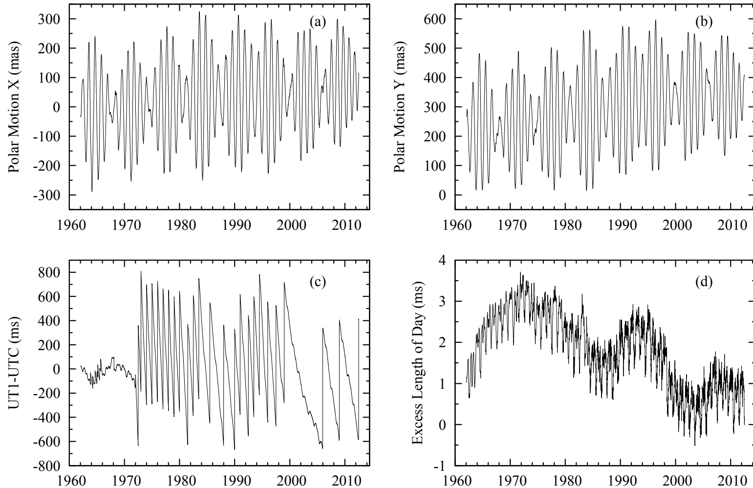
Figure 4. Plots of the x -component of polar motion (4a), y -component of polar motion (4b), UT1–UTC (4c), and excess length-of-day (4d) as given by the combined Earth orientation series, COMB2011. The discontinuous changes in the plot of UT1–UTC are caused by the presence of leap seconds. Prior to the introduction of leap seconds in 1972, Coordinated Universal Time (UTC) was adjusted by introducing step and rate changes designed to keep it close to UT1 (e.g., IERS 1997, Table II-3), the effect of which is also readily apparent in (4c). Note that the UT1–UTC values displayed in (4c) include the tidal variations, whereas the excess length-of-day values shown in (4d) do not.
