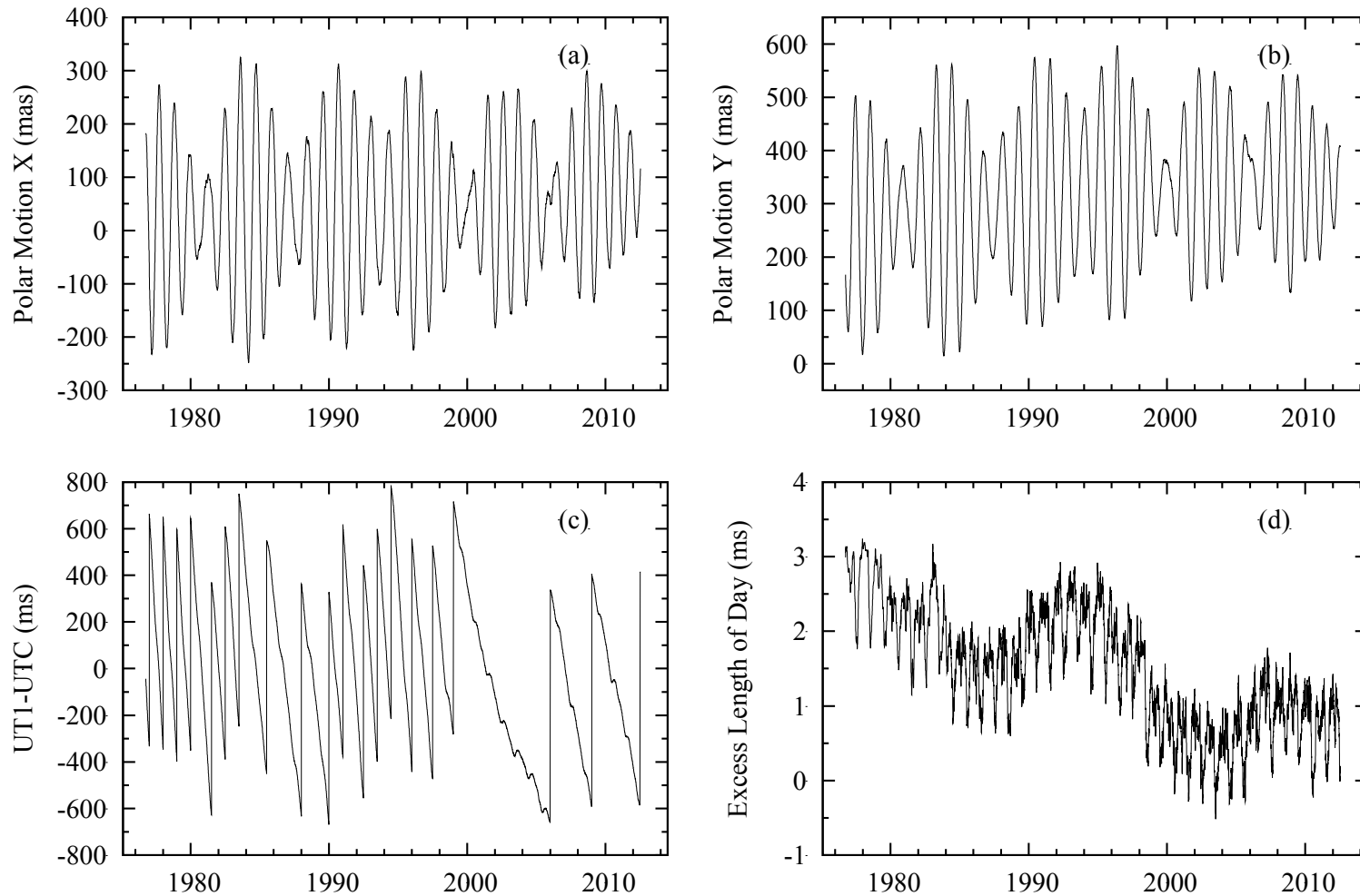
Figure 1. Plots of the x -component of polar motion (1a), y -component of polar motion (1b), UT1–UTC (1c), and excess length-of-day (1d) as given by the combined Earth orientation series SPACE2011. The discontinuous changes in the plot of UT1–UTC are caused by the presence of leap seconds. Note that the UT1–UTC values displayed in (1c) include the tidal variations, whereas the excess length-of-day values shown in (1d) do not.
