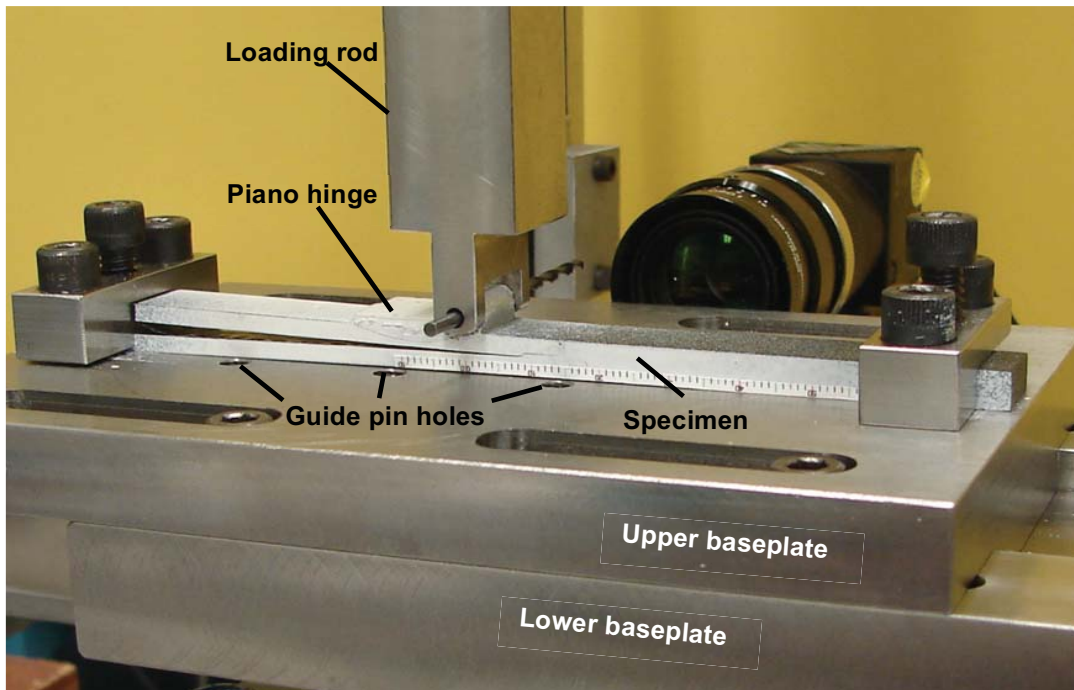
Figure 4. Delamination migration test fixture with loaded specimen (L=1.1a 0 ).
