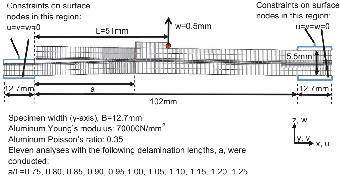
Figure 5. Finite element mesh of a specimen (mesh along z-axis expanded to aid view).
