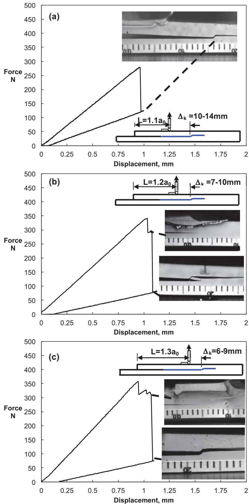
Figure 9. Force/displacement response of specimens (a) L=1.1a_0 , (b) L=1.2a_0 , (c) L=1.3a_0 .
