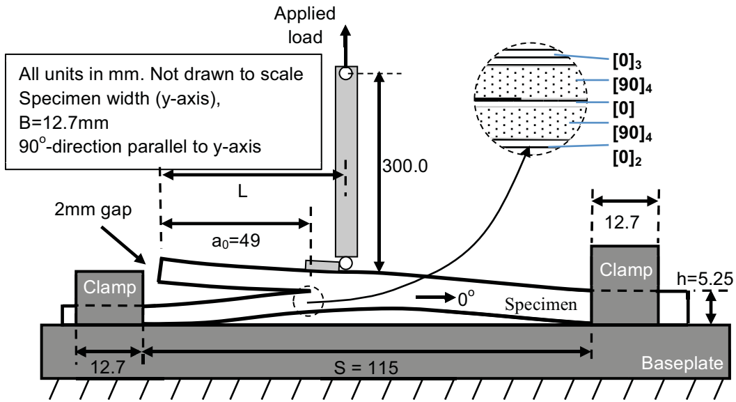
Figure 1. Schematic of delamination migration specimen.
