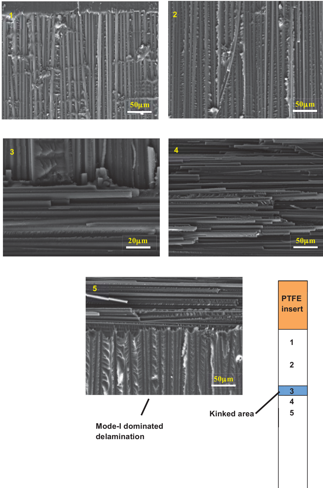
Figure 11. Scanning electron micrographs of specimen fracture surfaces ( L=1.3a_0 ).
