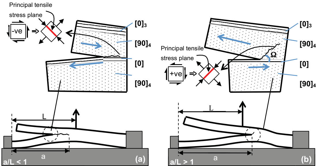
Figure 2. Shear stresses acting across the delamination front at different stages of a test.
