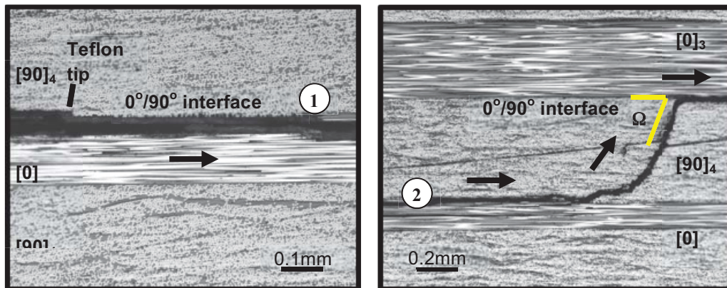
Figure 8. Micrographs of delamination onset and migration regions in a specimen.
