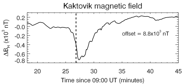
Figure 3. Ground-based magnetometer H (magnetic north) component at Kaktovik, Alaska. The vertical dashed line indicates the time at which GEODESIC was magnetically conjugate. After Burchill et al. [2004].
