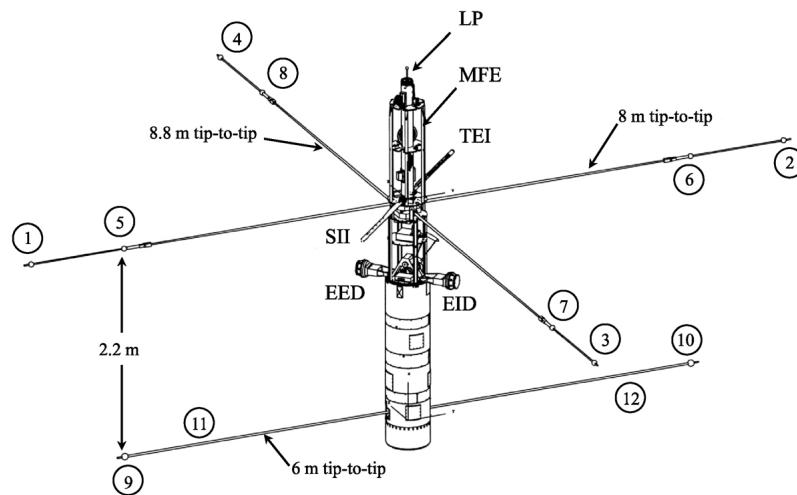
Figure 1. Payload configuration, showing the placement of the electric field spheres (numbered), Langmuir probe (LP), search coil antennas (MFE), Suprathernal Electron Imager (SII), Thermal Electron Imager (TEI), and the Energetic Electron and Ion Detectors (EED and EID). The payload was aligned with the geomagnetic field to within 5^\circ throughout most of the flight.
