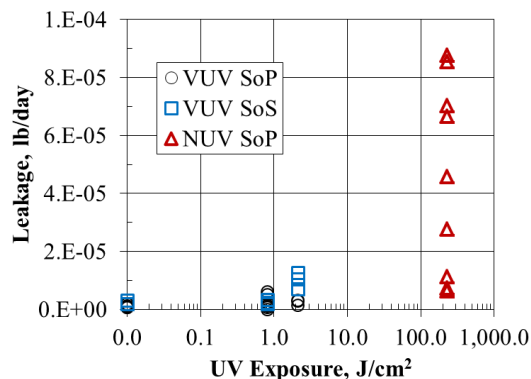
Figure 5.—Leakage of S0383-70 after exposure to VUV and NUV radiation.
