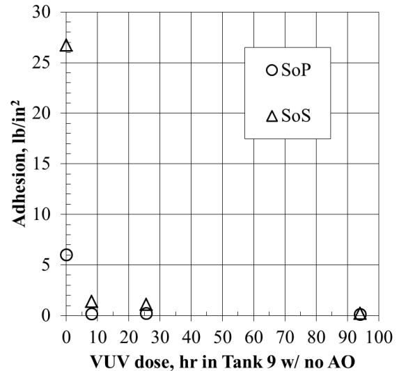
Figure 2.—Seal-on-Plate and Seal-on-Seal average adhesion of VUV exposed buttons, zero AO.
