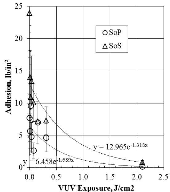
Figure 3.—Seal-on-Plate and Seal-on-Seal average adhesion of S0383-70 after VUV exposure in the 30-W lamp facility.
