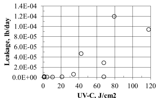
Figure 6.—Leakage of S0383-70 after exposure to UV-C radiation.
