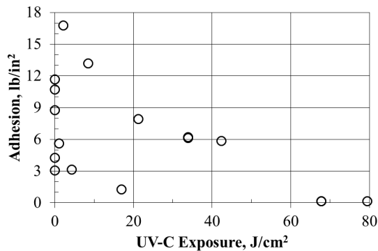
Figure 4.—Seal-on-Plate adhesion of buttons exposed to UV-C.
