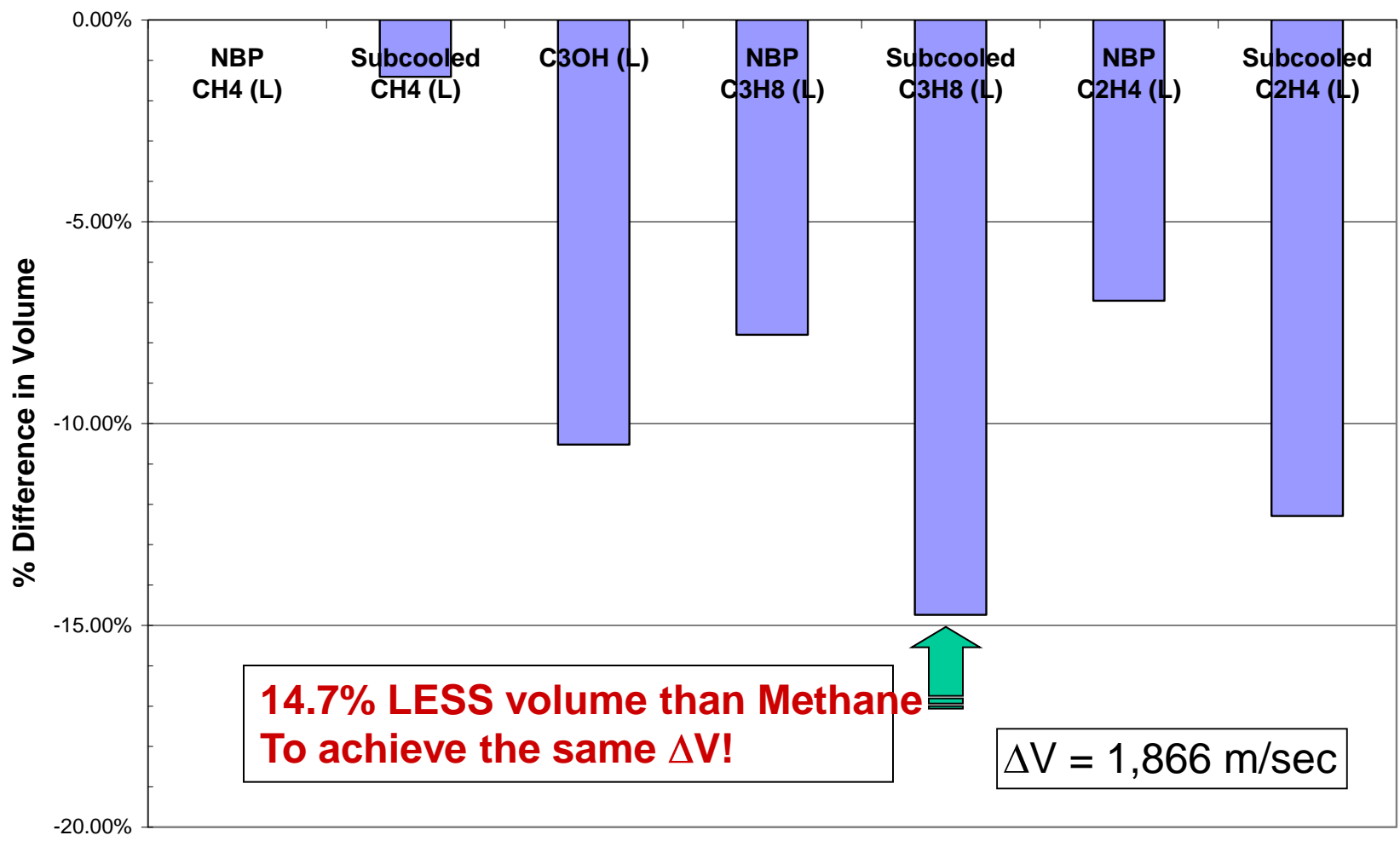
Propellant Tank Volume Comparison with LOX/Methane System
