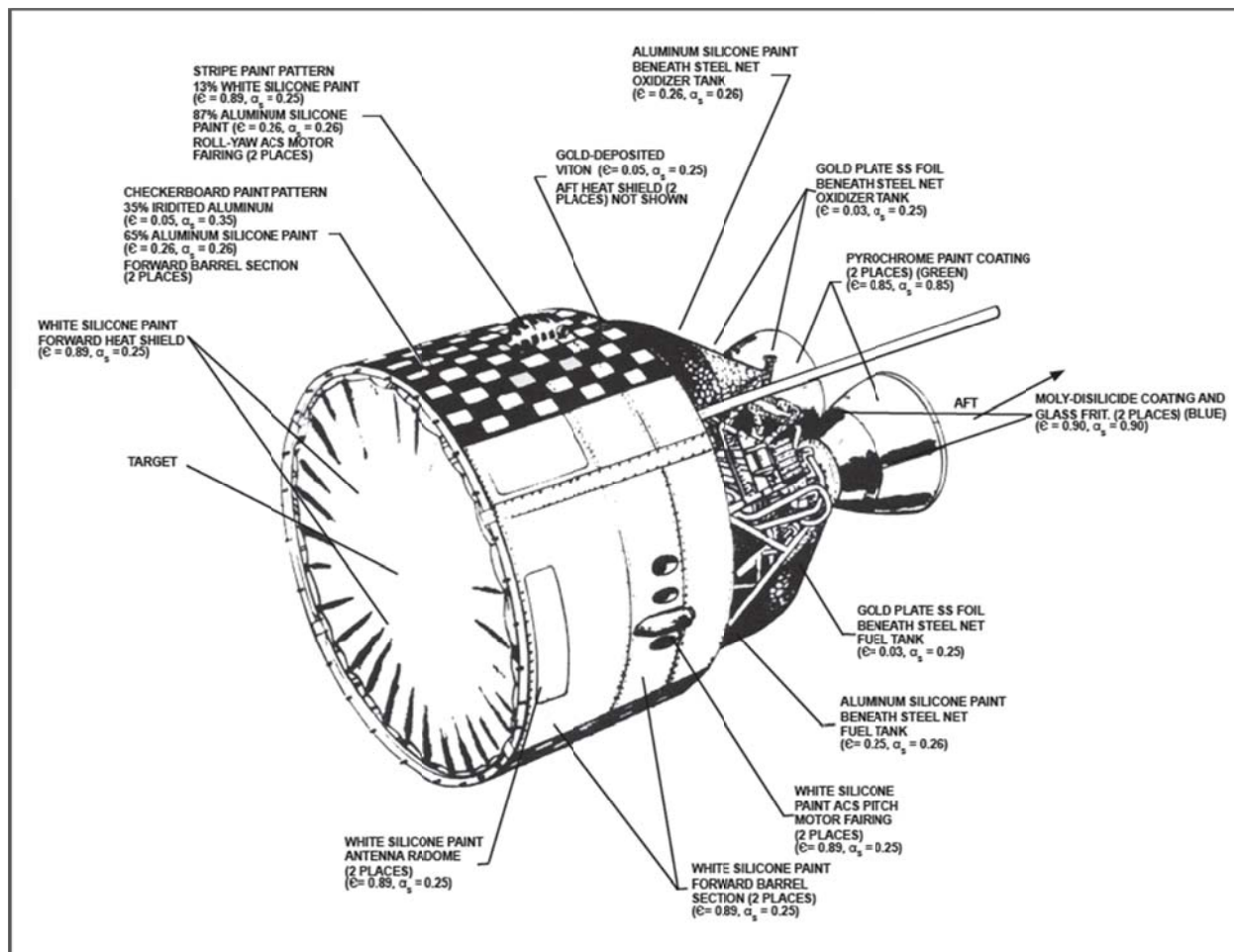
Fig. 1. Titan Transtage Schematic [2].
