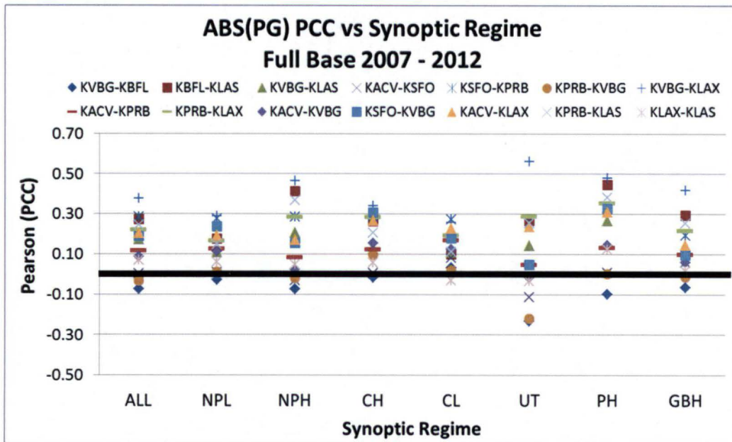
Figure 13. ABS(PG) PCC versus synoptic regime for the full base from 2007-2012. The solid black line highlights where PCC equals zero. The PCC is on the y-axis and the synoptic regime on the x-axis. The "ALL" category on the x-axis includes all of the days in the 2007-2012 database regardless of synoptic regime and the solid black horizontal line highlights where PCC equals zero.
