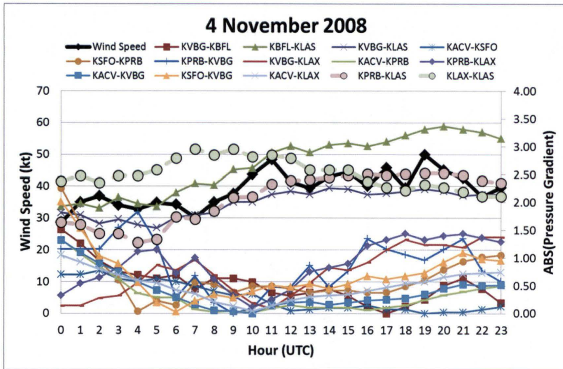
Figure 7. Same as Figure 5, except for 4 November 2008 in the NPL regime.
