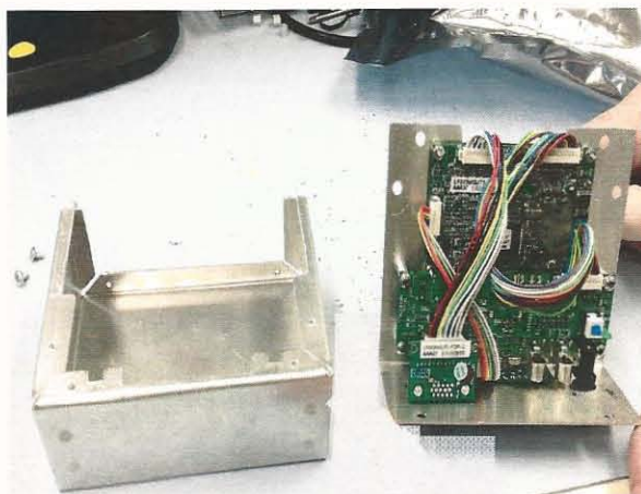
Figure 2 AMOLED Assembly Installed into Enclosure's Upper Lid
