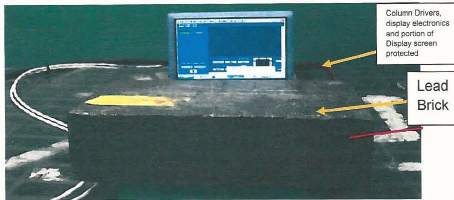
Figure 27 AMOLED with Radiation Shielding
