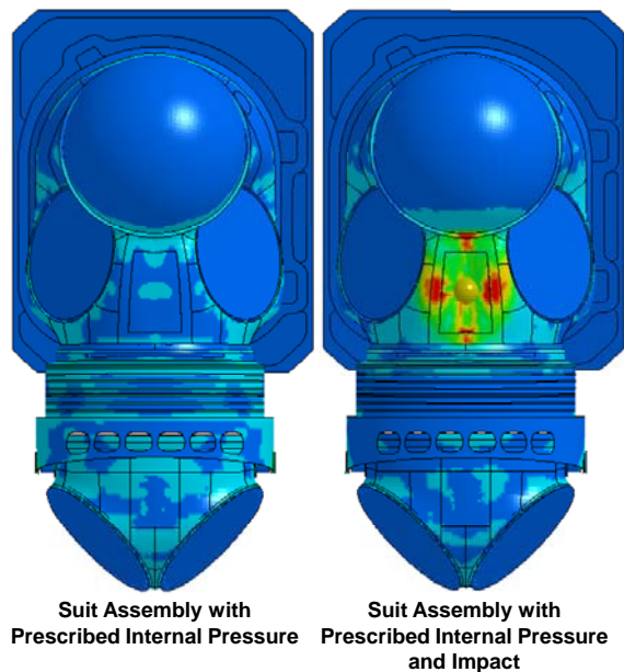
Figure 5: Arbitrary Stress Contours of the Space Suit Assembly with Prescribed Internal Pressure and Impact Loading Conditions.
