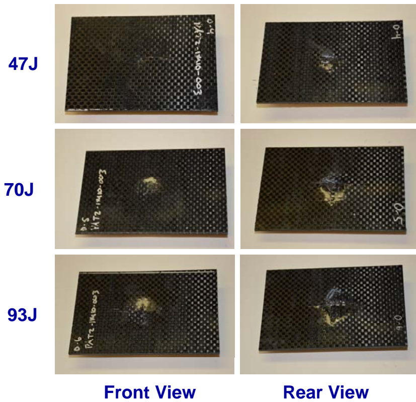
Figure 4: Low Velocity Impact Test samples for IM-10
