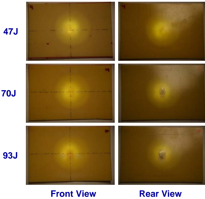
Figure 3: Low Velocity Impact Test samples for S-Glass
