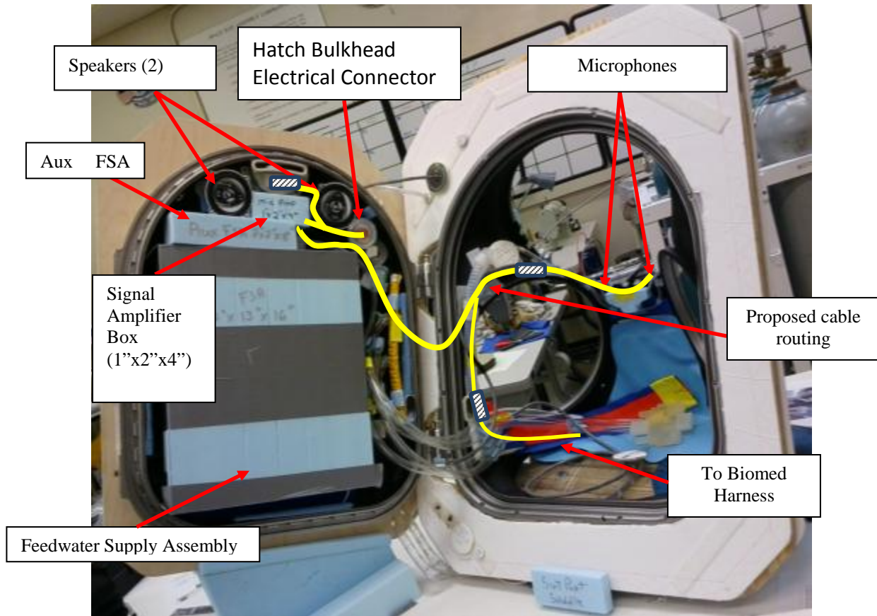
Figure 6: Examples of PLSS and PAS interfaces
