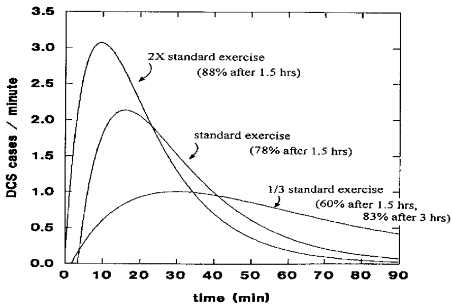
Figure 5. The rate of DCS as a result of exercise after an ascent to 3.0 psia without PB. Standard exercise was 10 step-ups on a 9-in stool in 30 sec, repeated at 5-min intervals.
