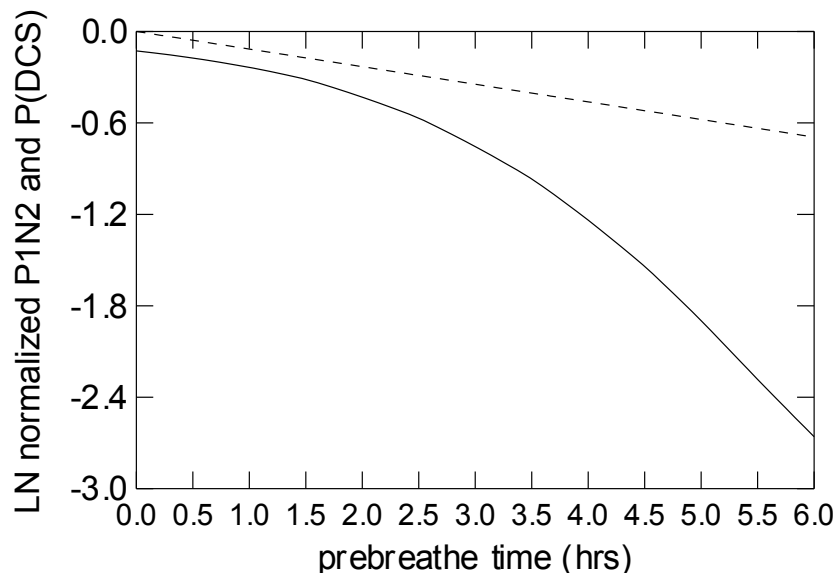
Figure 6. Change in computed tissue N_2 pressure (dashed curve) and the P(\text{DCS}) (solid curve) as a function of PB time under conditions of the simulation described in the text.
