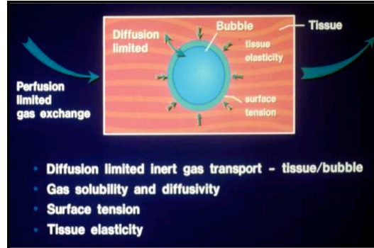
Figure 2. Tissue Bubble Dynamic Model equation and parameters
