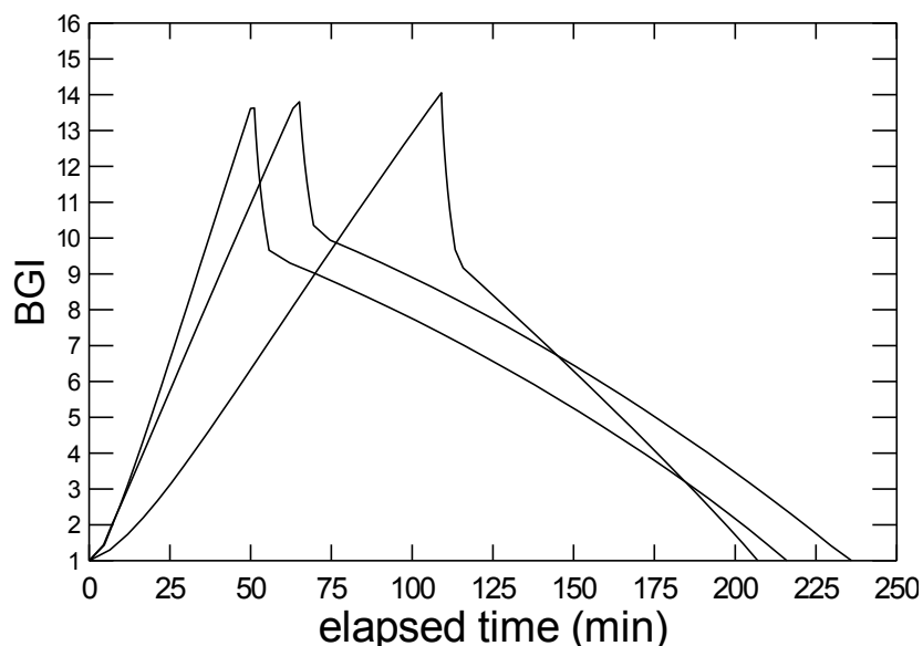
Figure 14. The resolution of a 14-unit BGI given a Boyle's Law decrease in bubble volume with applied treatment pressure and the bubble-to-tissue N_2 gradient. The first curve from the left is derived from data obtained after a 60-min PB in an astronaut exposed to 4.3 psia with return to 14.7 psia; the second curve represents data from a saturation diver with return to 41.1 psia after exposure to 14.7 psia; and the third curve is derived from data obtained after a 300-min PB in an astronaut exposed to 4.3 psia with return to 14.7 psia (5 min for all pressure transitions).
