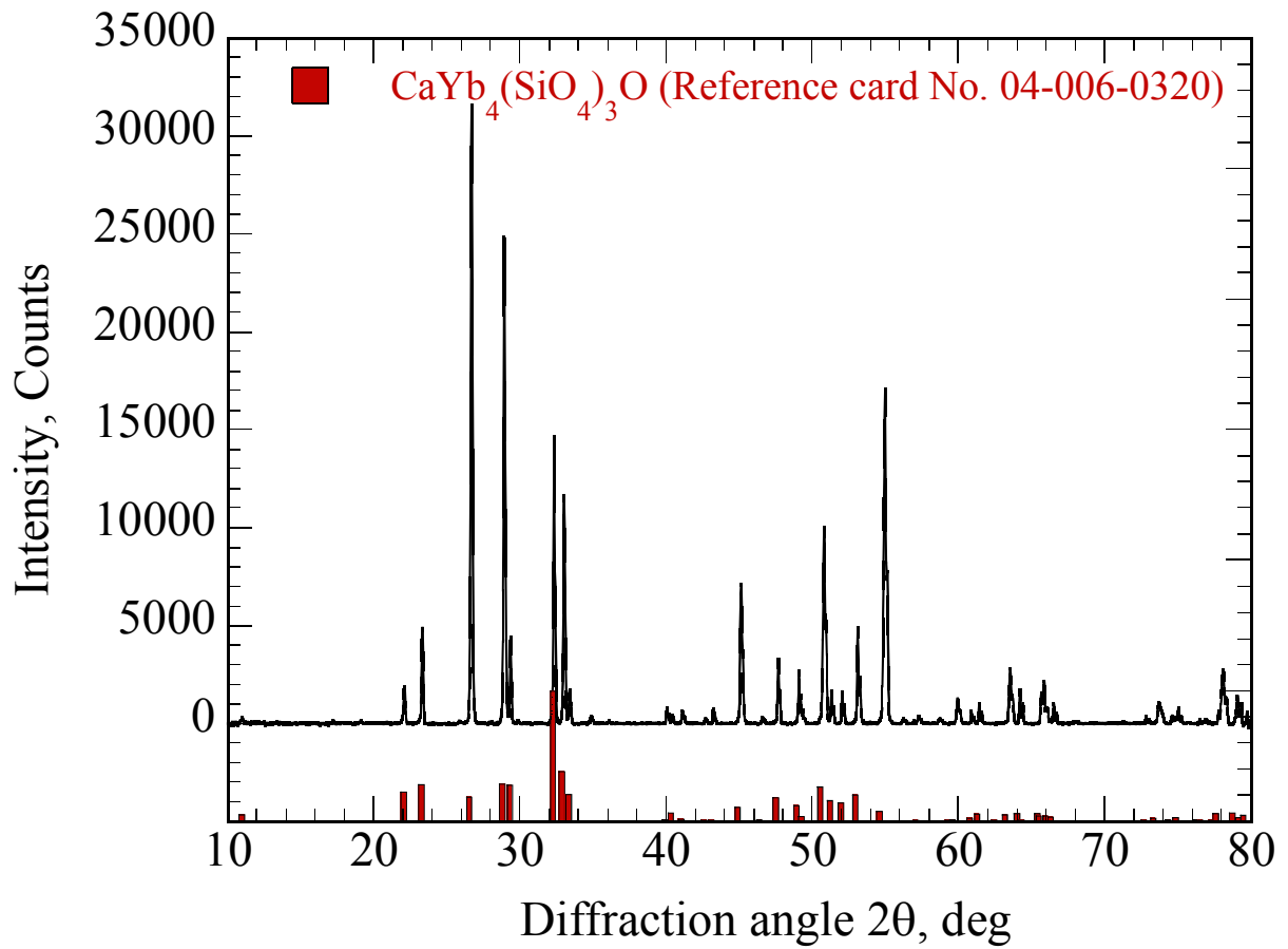
Figure 5.—XRD of \text{Yb}_2\text{SiO}_5 -CMAS reaction layer. The pattern for \text{Ca}_2\text{Yb}_8(\text{SiO}_4)_6\text{O}_2 matches well with the observed x-ray scan for the \text{Yb}_2\text{SiO}_5 -CMAS reaction layer.
