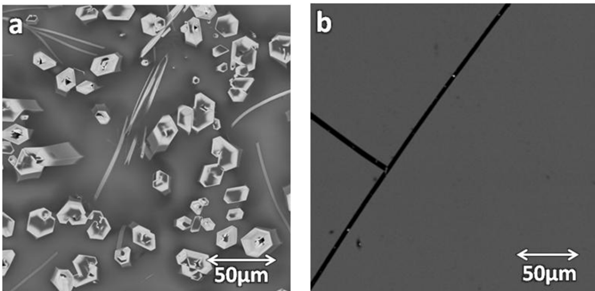
Figure 6.— \text{Yb}_2\text{SiO}_5 surface reacted with CMAS for (a) 5 h at 1500 °C and (b) 50 h at 1300 °C.
