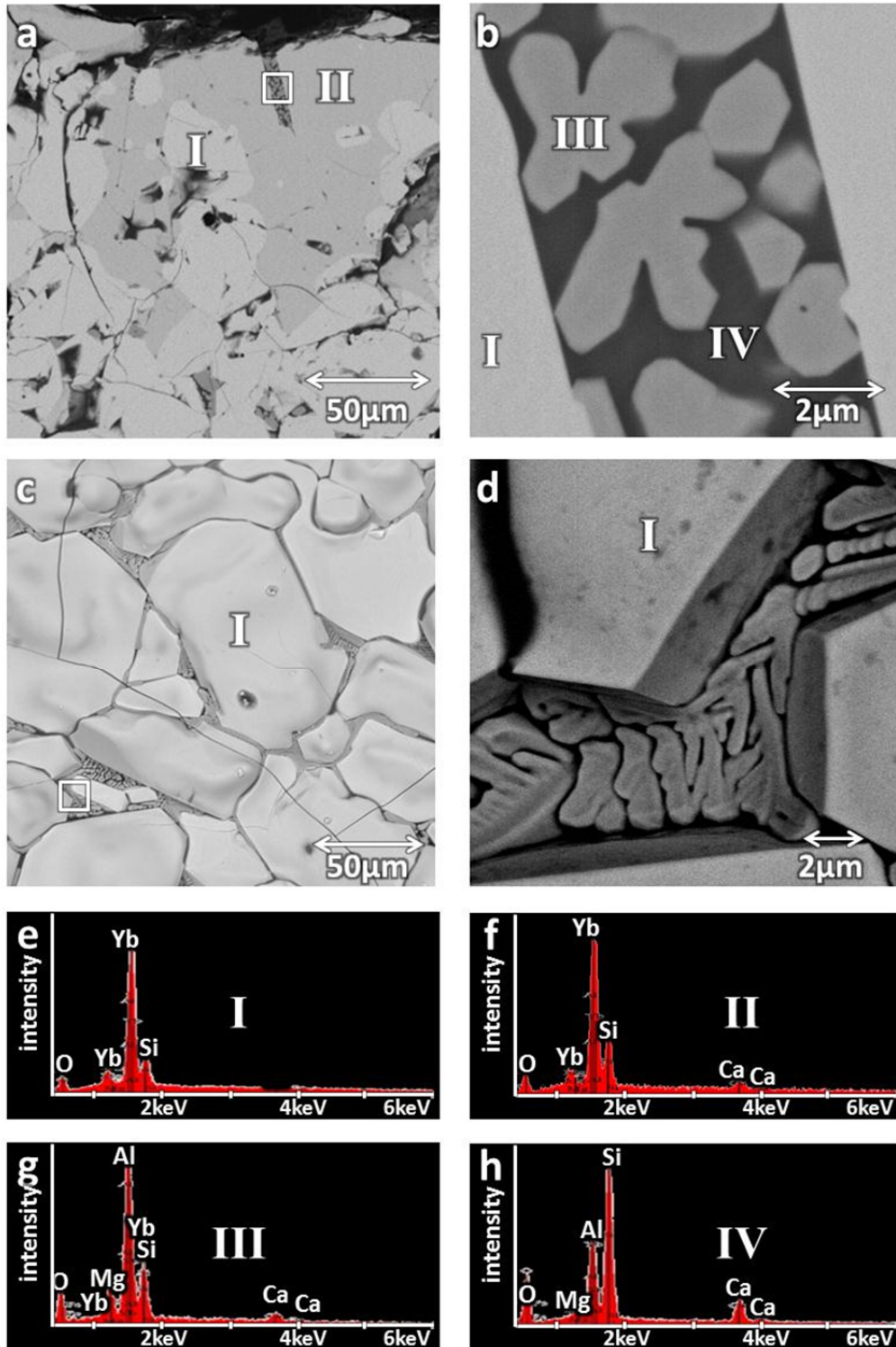
Figure 4.—SEM images of \text{Yb}_2\text{SiO}_5 reacted with CMAS for 200 h. (a), (b), (c), and (d) low and high magnification surface BSE images of \text{Yb}_2\text{SiO}_5 reacted with CMAS for 200 h at 1500 °C; and (e) and (h) EDS of regions I-IV, respectively.
