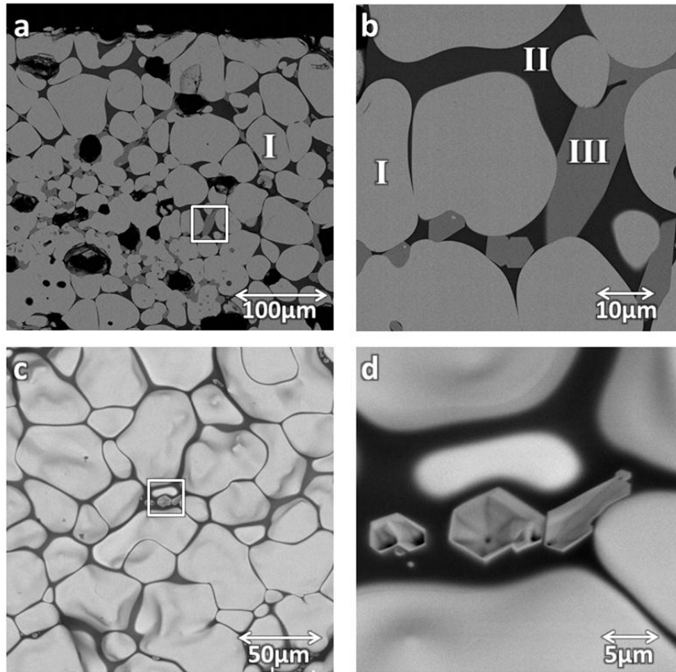
Figure 13.— \text{HfO}_2 reacted with CMAS for 100 h. (a) and (b) Low and high magnification cross-sectional images of RE-oxide doped \text{HfO}_2 reacted with CMAS for 100 h at 1500 °C; (c) and (d) Low and high magnification surface BSE images of RE-oxide doped \text{HfO}_2 reacted with CMAS for 100 h at 1500 °C. Similar to the rare earth silicate cases, the high concentration rare earth doped \text{HfO}_2 had relatively substantial grain boundary recessions and CMAS reaction phases.
