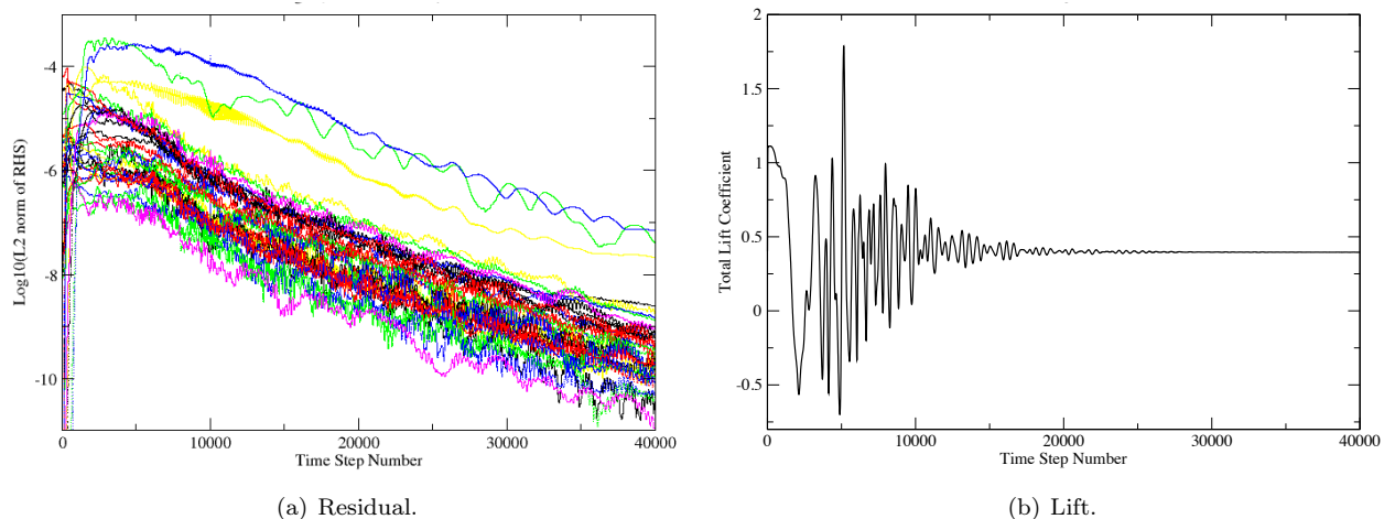
Figure 9: A typical convergence in Overflow.
