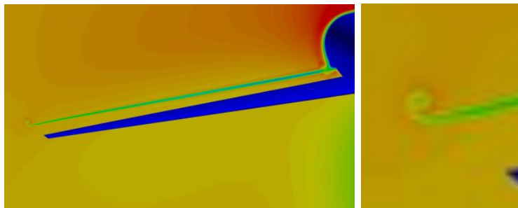
(b) Planar cut behind the wing showing the tip vortex. (c) Zoom-in view of the tip vortex.
