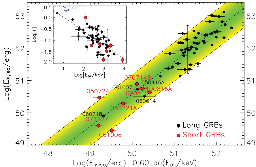
Figure 10. Three parameter correlation involving E_{X,\text{iso}} , E_{\gamma,\text{iso}} and E_{\text{pk}} . Dashed line: best-fitting relation (Eq. 8); dot-dashed lines mark the 95% confidence area around the best-fitting law. Notably, long and short GRBs share the same scaling, with short and sub-energetic GRBs (like GRB 060218) occupying the same area of the plot. Inset: evolution of the efficiency parameter \epsilon \equiv E_{X,\text{iso}}/E_{\gamma,\text{iso}} as a function of the spectral peak energy of the prompt emission E_{\text{pk}} . A reference \epsilon \propto E_{\text{pk}}^{-0.6} scaling has been marked with a blue dashed line.
