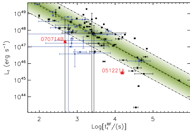
Figure 7. Luminosity at the end of the plateau phase, 0.3-30 keV (rest-frame) vs. end-time of the plateau. Colour coding as in Fig. 6. Blue points are for type Ia LCs.
