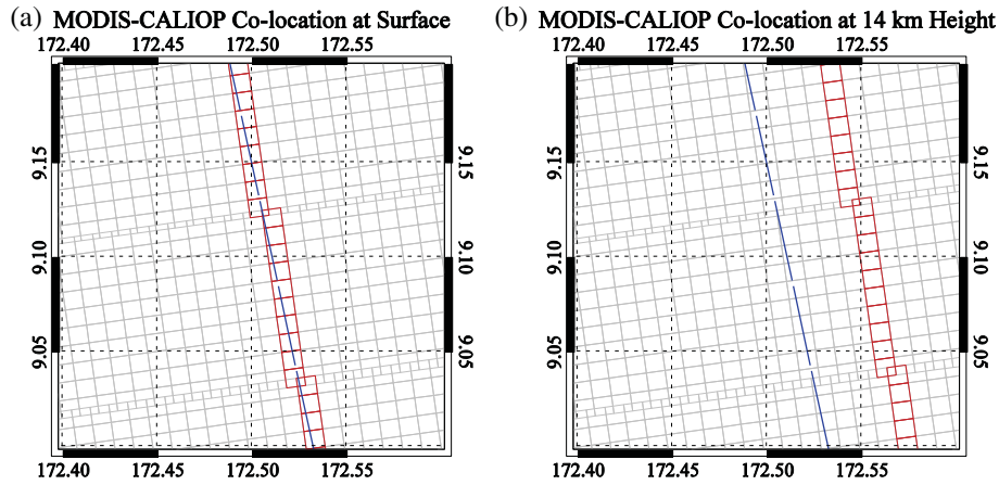
Figure 5. An example of collocated MODIS and CALIOP footprints at (a) surface and (b) 14 km height. Blue lines represent CALIOP foot prints in 5 km resolution, and red boxes collocated MODIS pixels in 1 km pixel resolution. There are at maximum five collocated MODIS pixels corresponding to a single CALIOP footprint.
