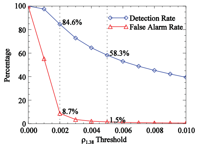
Figure 6. Cirrus detection rate and false alarm rate of MODIS with respect to \rho_{1.38} threshold values in reference to the cirrus detection from CALIOP over the eastern tropics ( 60^{\circ}\text{E} – 180^{\circ}\text{E} , 15^{\circ}\text{S} – 15^{\circ}\text{N} ) for the period from 1 March 2007 to 31 May 2007. The total numbers of data points for the cirrus-detected and clear cases determined by CALIOP are 105,548 and 54,243, respectively.
