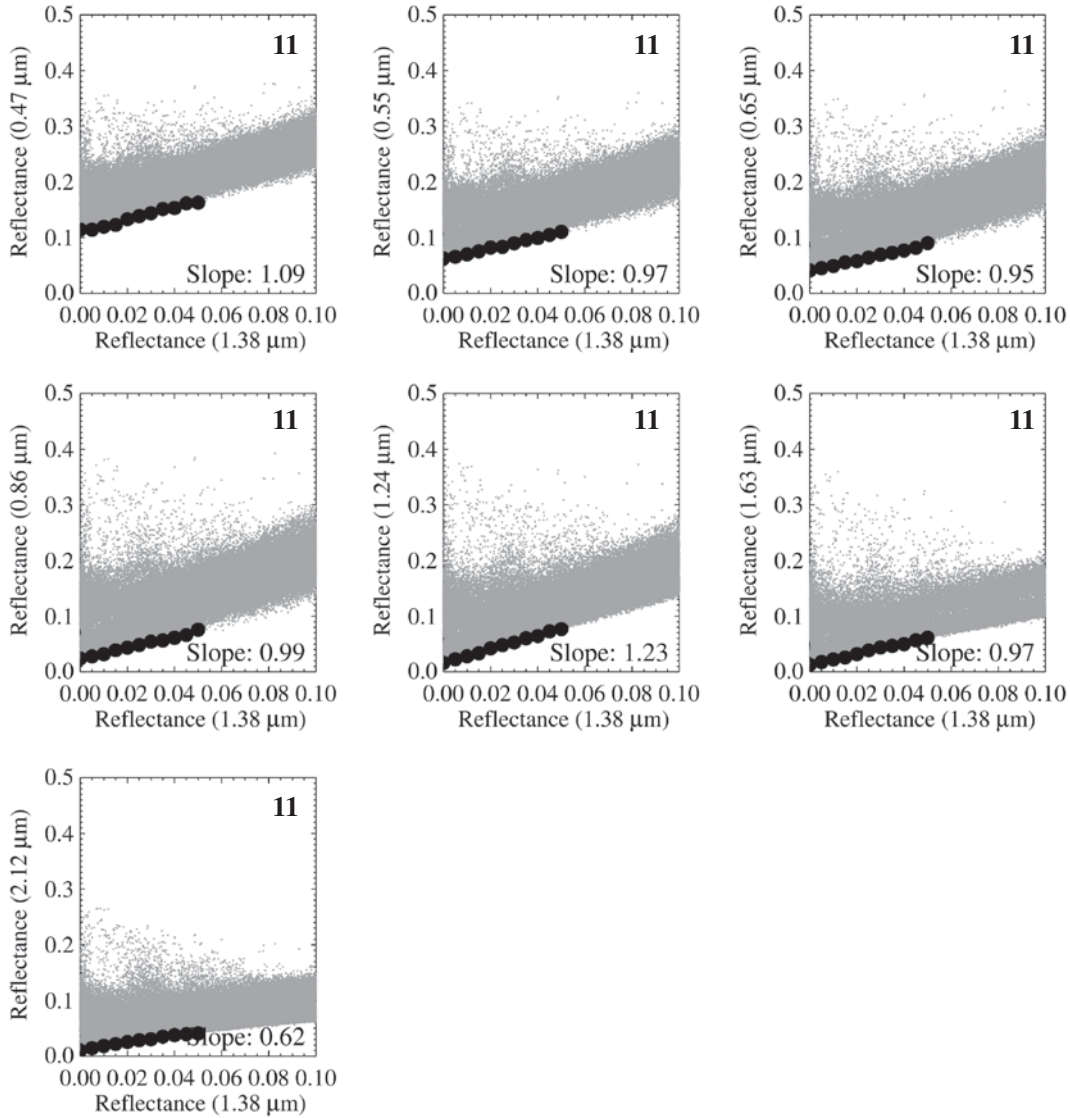
Figure 4. Spectral scatterplots between TOA reflectance at 1.38 μm and aerosol bands at number 11 corner point where cirrus clouds are observed.
