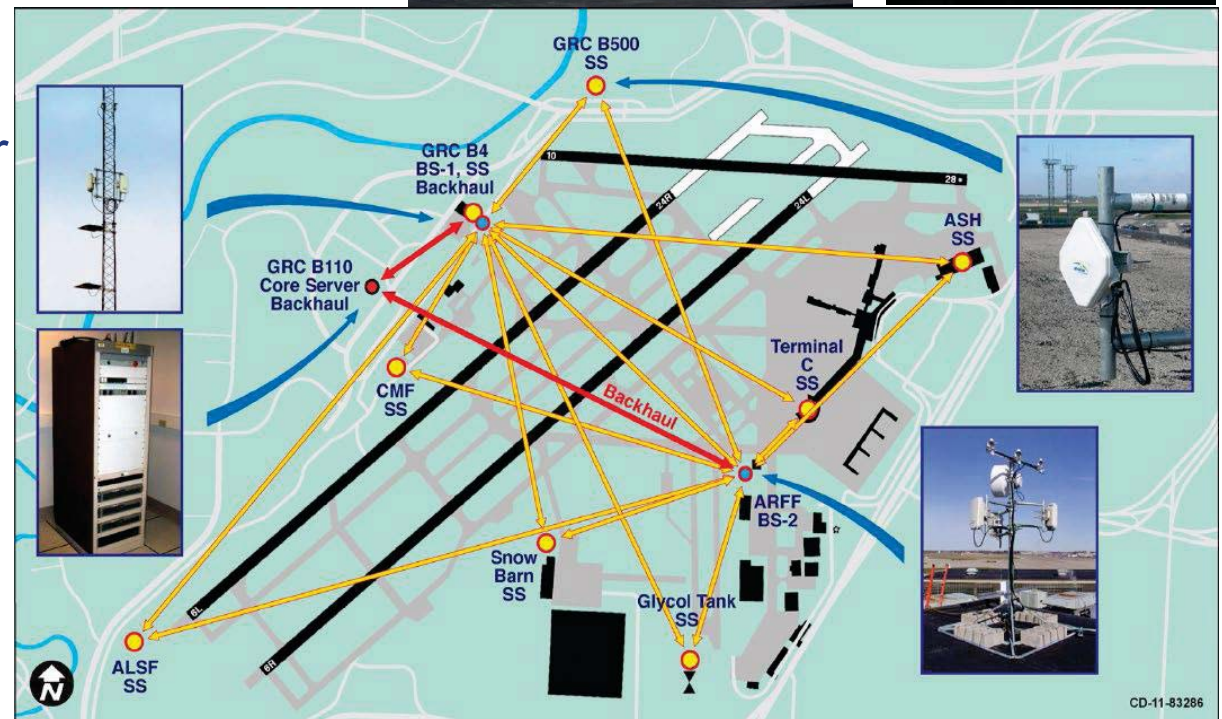
NASA-CLE CNS Test Bed AeroMACS Configuration
