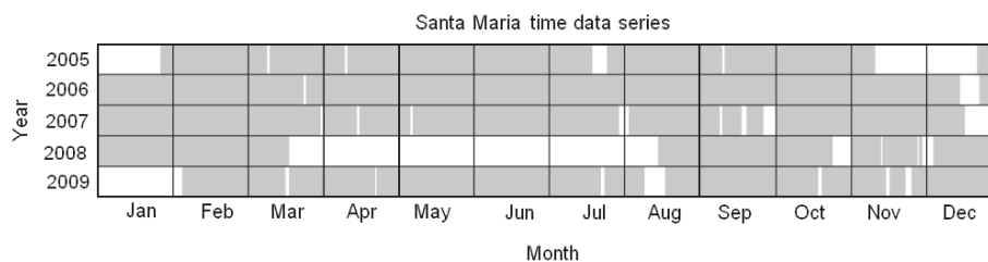
Fig. 3. The same as Fig. 1 but for the meteor radar at SM.
