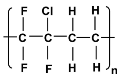
Figure 1: Halar molecular structure and an image of a cut Halar coated stainless steel sample coupon used for testing.
