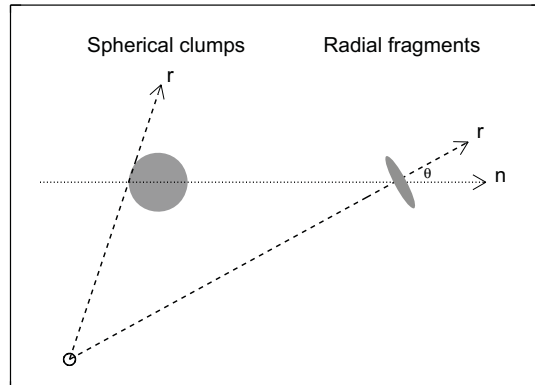
Figure 1. Schematic of photon of direction \mathbf{n} impacting a spherical clump and a radially oriented ( \mathbf{r}/|r| ) shell fragment. The former gives an isotropic effective opacity whereas the latter gives an anisotropic effective opacity, since the projected surface area depends on direction cosine \mu \equiv \cos \theta = \mathbf{n} \cdot \mathbf{r}/|r| .
