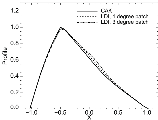
Figure 6. Line profiles for \tau_* = 2.5 , calculated from a smooth CAK model and structured LDI models with patch sizes 1 and 3 degrees (see text), as labelled.
