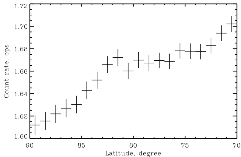
Figure 2. Latitude profile of counting rate averaged over 1^\circ latitudinal belts for North polar region. Statistical uncertainties are shown as vertical error bars.
