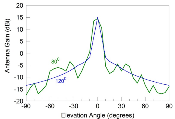
Figure 1. Modeled Gain versus Elevation Angle for AeroMACS Antennas
